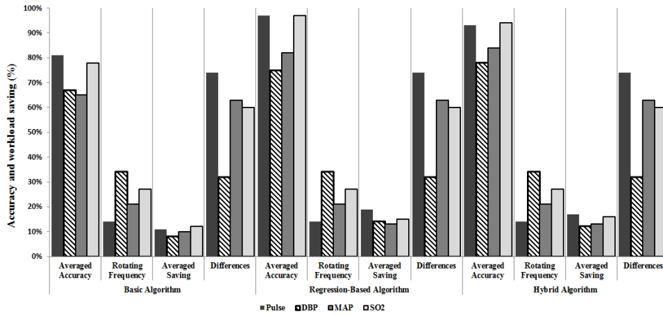
Fig. 6. Rotating Frequency Analysis for each Algorithm under four Measurements
