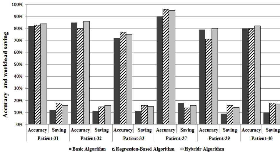
Fig. 7. Comparison the Performance of the Three Algorithms for each Patient
