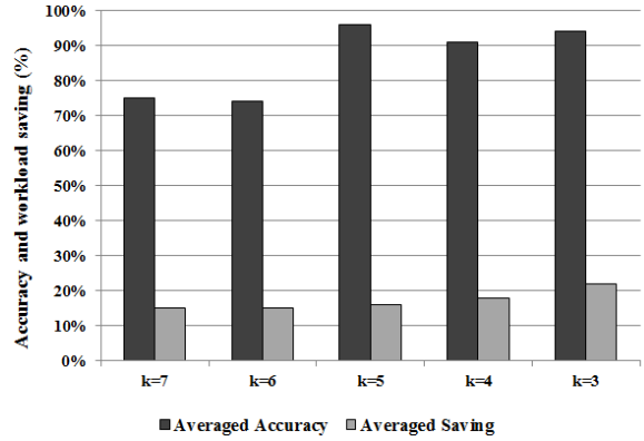
Fig. 2. The Averaged Accuracy and Workload Savings for all algorithms under Varying Values of k
