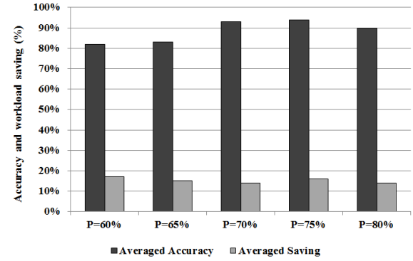
Fig. 3. The Averaged Accuracy and Workload Savings for all algorithms under Varying Values of p
