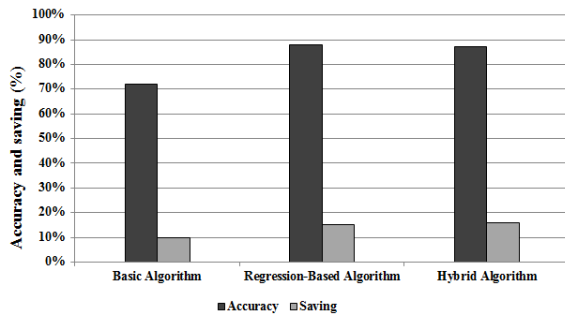
Fig. 5. Average Accuracy and Workload Saving for Each Algorithm
