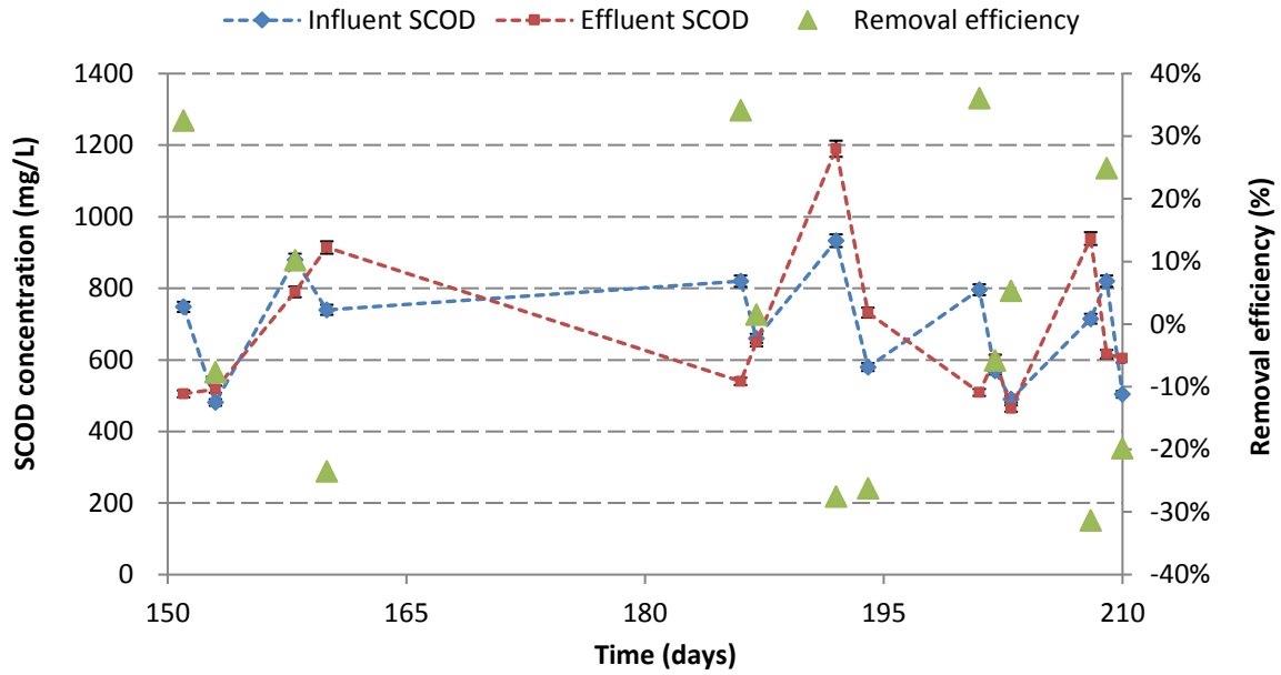
Figure 4. Evolution of MLSS (top), TCOD (middle) and SCOD (bottom) and the respective removal efficiency during continuous operation of the A-stage process with \text{Fe}^{3+} dosage (tests 7 to 10). Error bars indicate standard deviation. The error bars were omitted when smaller than the marker.
