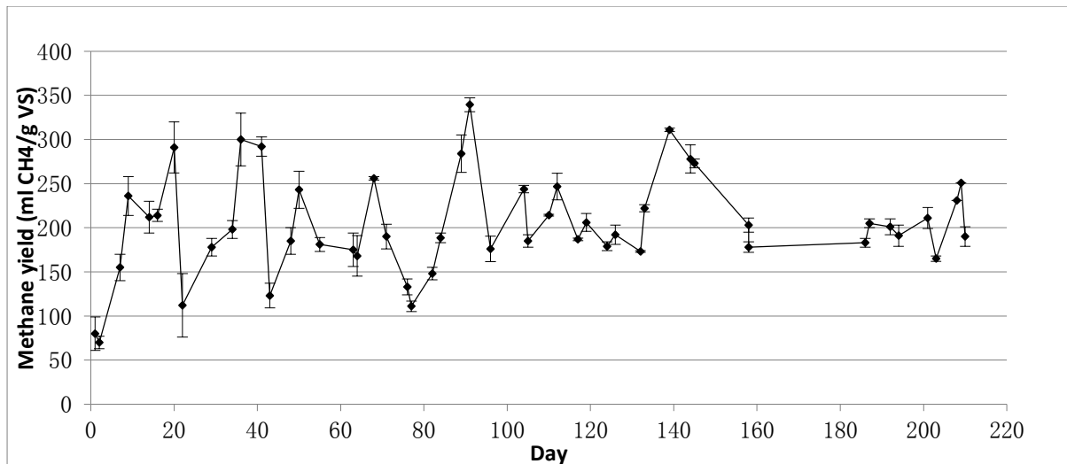
Figure 7. Methane yield of spent sludge. Error bars indicate the standard deviation.
