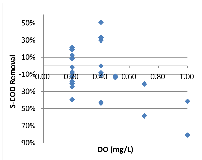
Figure 3. Effect of Dissolved Oxygen on SCOD removal percentage at DO in the range 0.2-1 mg/L (tests 1 to 6).
