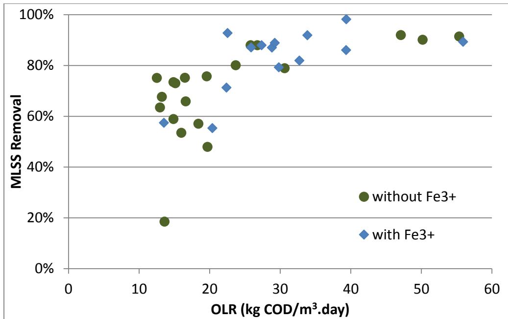
Figure 6. Effect of the Organic Loading Rate (OLR) on the MLSS removal with and without Fe 3+ dosage (all data point in tests 1 to 10).
