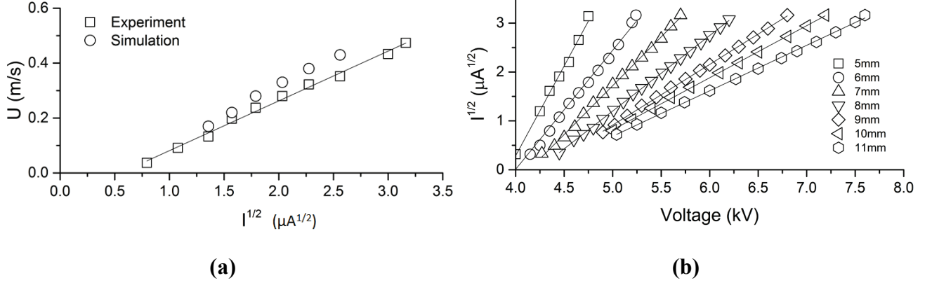
Fig. 3. Results for pin tip SR = 80 \mu\text{m} . (a) The ion wind velocity plotted with \sqrt{I} for electrode separation of 6 mm. (b) The \sqrt{I} plotted with the discharge voltage V for a range of electrode separation from 5 to 11 mm.
