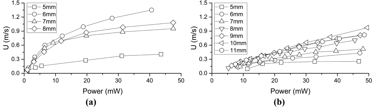
Fig. 4. Velocity of ion wind U plotted with the applied power with (a) pin tip SR = 15 \mu m and a range of electrode separations from 5 to 8 mm; and (b) pin tip SR = 80 \mu m and a range of electrode separations from 5 to 11 mm.
