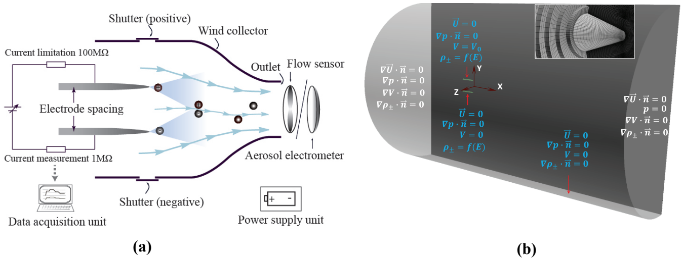
Fig. 1. Bipolar discharge ion wind generator. (a) Experimental setup. (b) Numerical simulation model, a cylindrical domain with diameter and length of ten and twenty times of electrode separation; the inset shows magnified view of mesh at pin tip.
