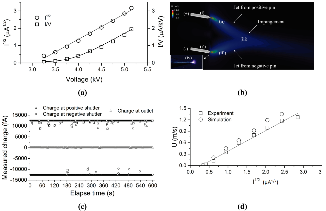
Fig. 2. Result for pin tip \text{SR} = 15 \mu\text{m} . (a) Voltage – current for electrode separation of 6 mm. (b) Velocity field simulation of the ion wind generation with parameters given in Fig. 2a. (i) & (i') pin tips; (ii) & (ii') jet of ion clouds; (iii) impingement point and (iv) glowing corona image taken at negative pin tip with applied voltage of 4.5 kV and discharge current of 4.0 \mu\text{A} . (c) Charge measurement results. (d) The ion wind velocity plotted versus \sqrt{I} .
