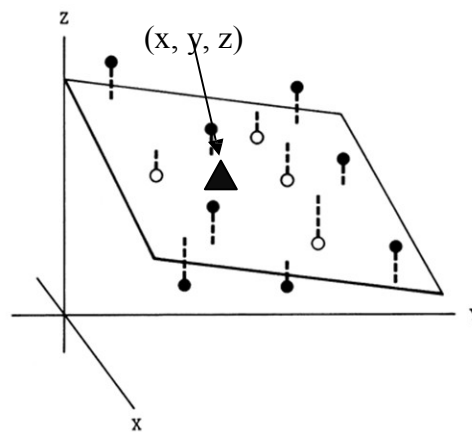
Fig. 2 – The z value (pixel intensity value) of the black triangle at a required grid intersection (x, y) coordinates is the value calculated on the least square plane determined by twelve adjacent pixel intensity values.
