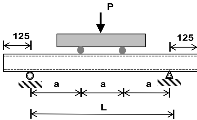
Figure 1. Experimental set-up for characterisation of elastic properties
