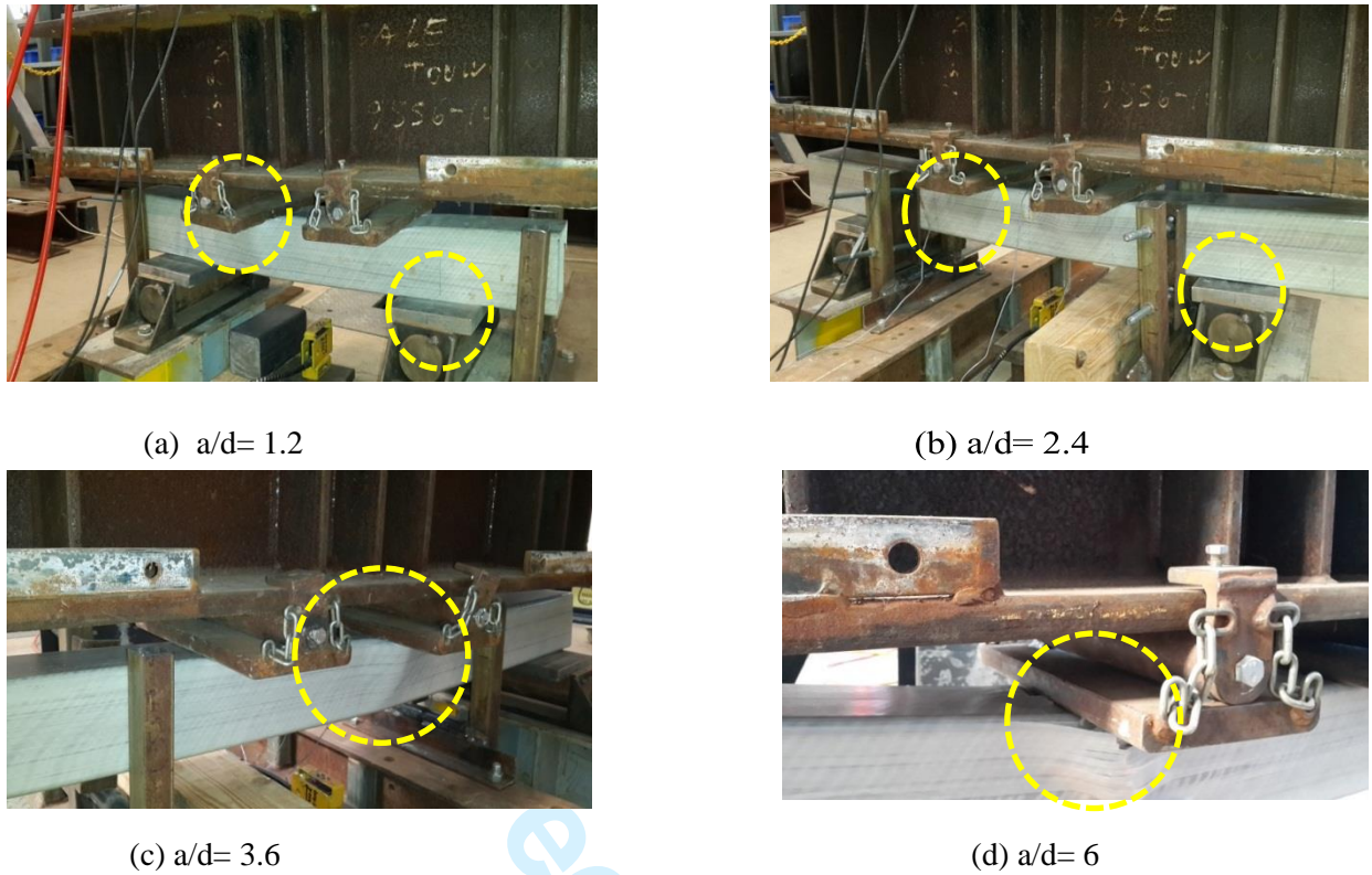
Figure 12. Failure modes of GFRP beams for different shear span to depth ratios
