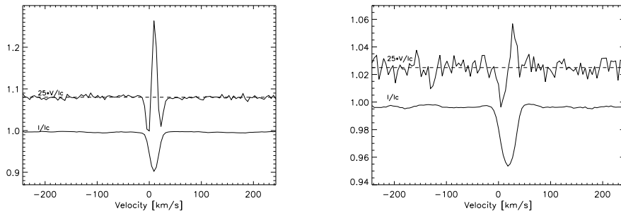
Figure 1. Stokes I and V Least-Squares Deconvolved line profiles of the Ap stars HD 43819 (left) and HD 171782 (right). Stokes V Zeeman signatures (magnified and shifted for display purposes) are clearly detected. Adapted from Aurière et al. (2007).
