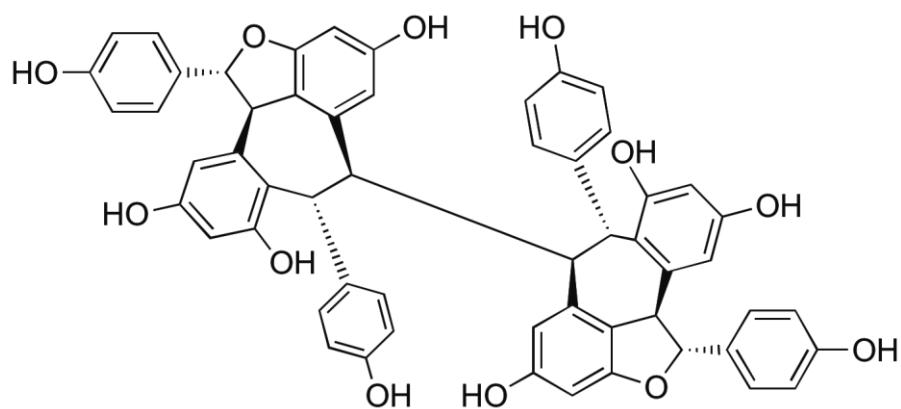
(-)-Hopeaphenol
