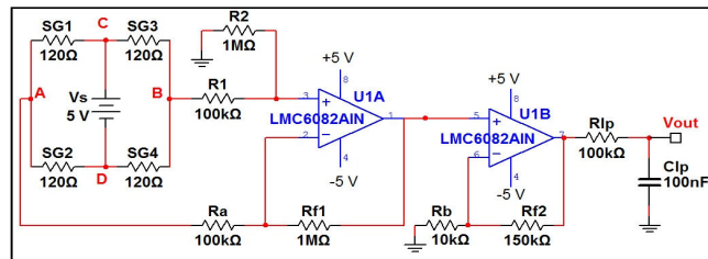
Fig. 2(a). Schematic Diagram of the Strain Gauges Sensor Circuit.
