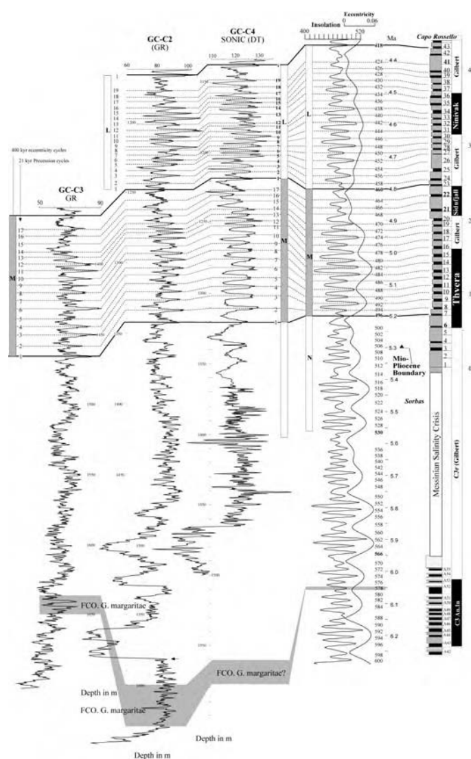
Fig. 3. Gamma ray (GR) and sonic (DT) logs for boreholes GC-C2, GC-C3 and GC-C4 drilled in the Gulf of Cadiz. Modified from Ledesma, 2000. Analysis of cycle patterns allowed the astrochronological correlation of these logs with the 65°N summer insolation record (Laskar et al. , 1990) and Capo Rossello section (after Hilgen, 1991; Langereis and Hilgen, 1991; Lourens et al. , 1996) in the Mediterranean (see Sierra et al. , 2000; Ledesma, 2000). For reference, rhythmic sections from the Sorbas basin are shown (Sierra et al. , 2001; Krijgsman et al. , 2001). Astronomical cycles are clearly recorded in the logs from nearly the base of the Pliocene. The Miocene-Pliocene transition is marked by a change in physical properties as recorded in the logs. Letters L, M, N mark the 400 kyr cycles as recognized in Sierra et al. , 2000 and in Ledesma, 2000).
