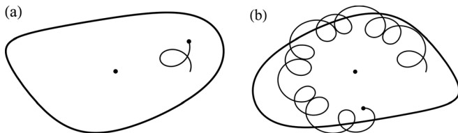
Fig. 5. Test particle orbit in the laboratory reference frame: (a) t = \pi/\Omega ; (b) t = 12 \pi/\Omega . The dot on the orbit marks the instantaneous position of the particle. The closed curve shows the instantaneous position of the solenoid wall. The central dot marks the rotation axis of the solenoid. Although a part of the trajectory image is outside the solenoid (at t = 12 \pi/\Omega ), the particle itself always stays inside of the solenoid.
