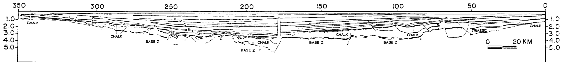
Figure 13b: A line drawing interpretation of NOPEC CNST-82 based on well information and seismic profiles. Note the mid-Jurassic through early Cretaceous faulting in the center of the profile indicating the Central Graben. Also note the continuity of the base Zechstein horizon either side of the Central Graben.
