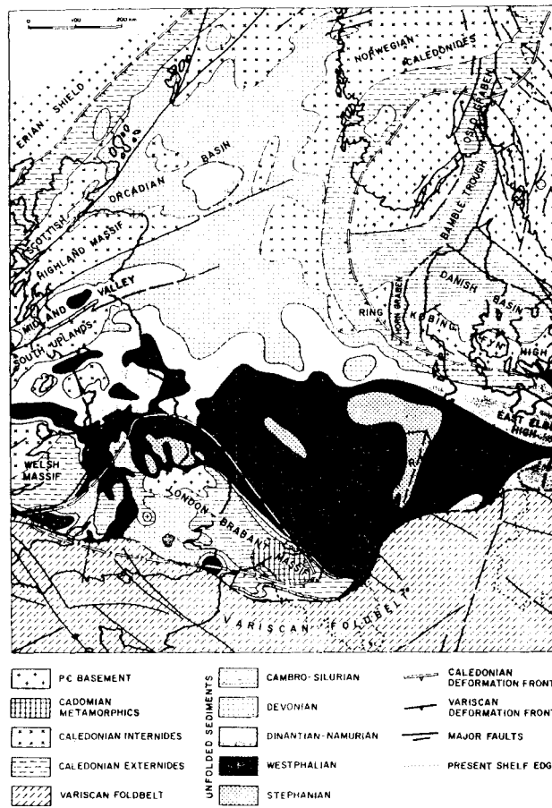
Figure 1a: Pre-Permian subcrop map of Northwestern Europe (Ziegler, in press).
