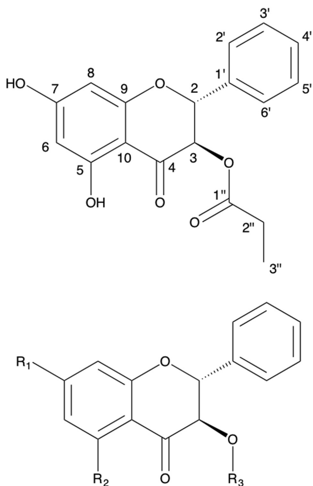
Fig. 1. Generalized flavonoid carbon numbering system.
