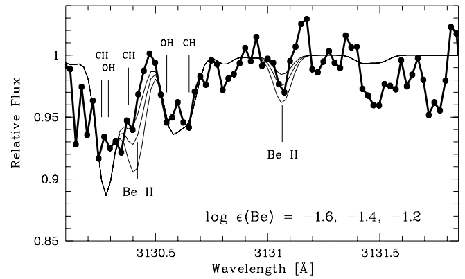
FIG. 12.—Spectral region ( connected dots ) of the two beryllium lines at \sim 3130 Å in HE 1327–2326. Synthetic spectra are overplotted ( solid lines ) for three Be abundances. The upper limit derived from both lines is \log \epsilon(\text{Be}) < -1.2 . [See the electronic edition of the Supplement for a color version of this figure.]
