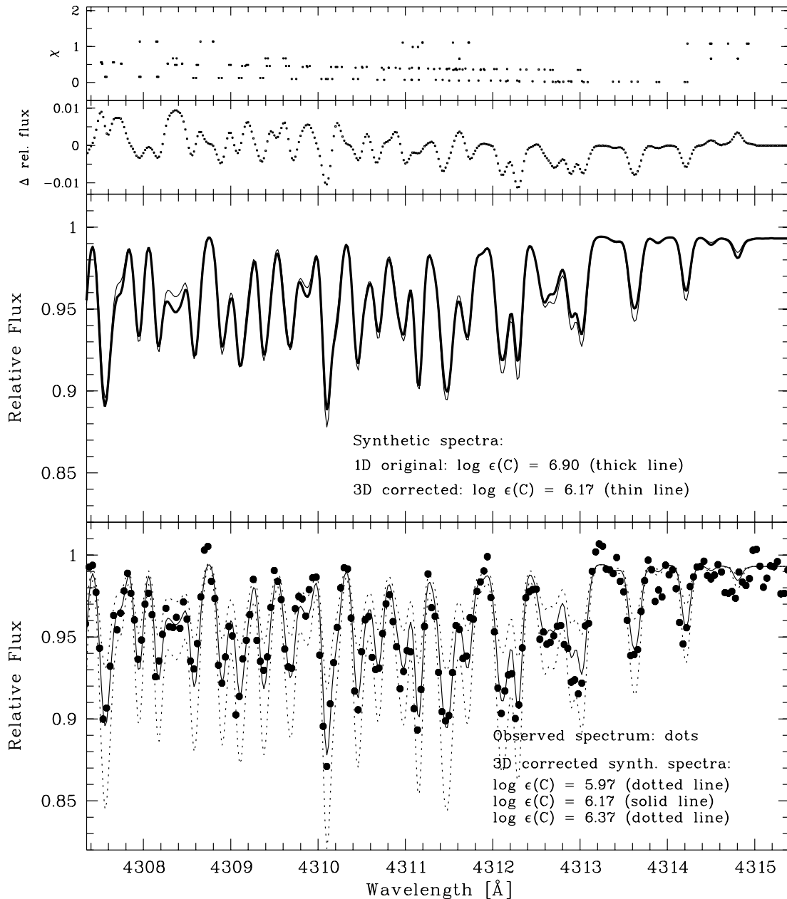
FIG. 8.—CH G-band spectral region of HE 1327–2326. Top : Excitation potentials of the molecular CH lines. Second from top : Flux difference between the “1D” and “3D-aided” synthetic spectra ( second panel from bottom ) is given. A comparison of the “1D” synthetic spectrum with a synthetic spectrum generated from the 3D-adjusted line list is shown in the second panel from the bottom. The abundance of the 3D-aided synthetic spectrum was varied to reproduce the 1D spectrum, and so the average difference of the two fluxes seen in the panel above becomes zero over the given wavelength range. Abundances are as given. Bottom : Observed Subaru HDS spectrum ( dots ) overplotted with 3D-aided synthetic spectra with C abundances of [C/Fe] = 3.78 ( solid line ), 3.58, and 3.98 ( dotted lines ). The average 3D–1D correction over this wavelength range for CH is -0.69 dex. [See the electronic edition of the Supplement for a color version of this figure.]
