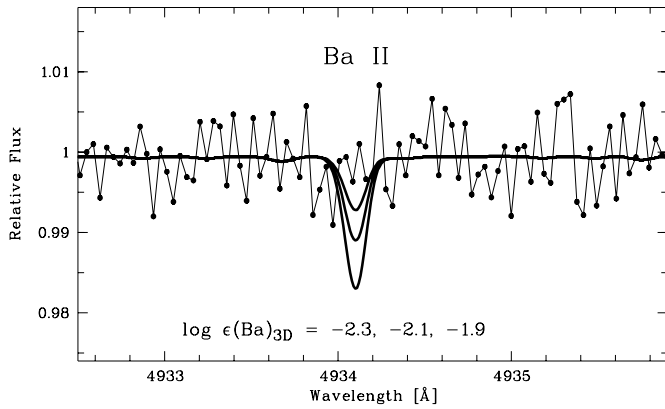
FIG. 15.—Spectral region ( connected dots ) of the barium line at 4937 Å in HE 1327–2326. Synthetic spectra are overlotted ( solid lines ) for three Ba abundances. The upper limit for this line is \log \epsilon(\text{Ba}) < -2.04 . [See the electronic edition of the Supplement for a color version of this figure.]
