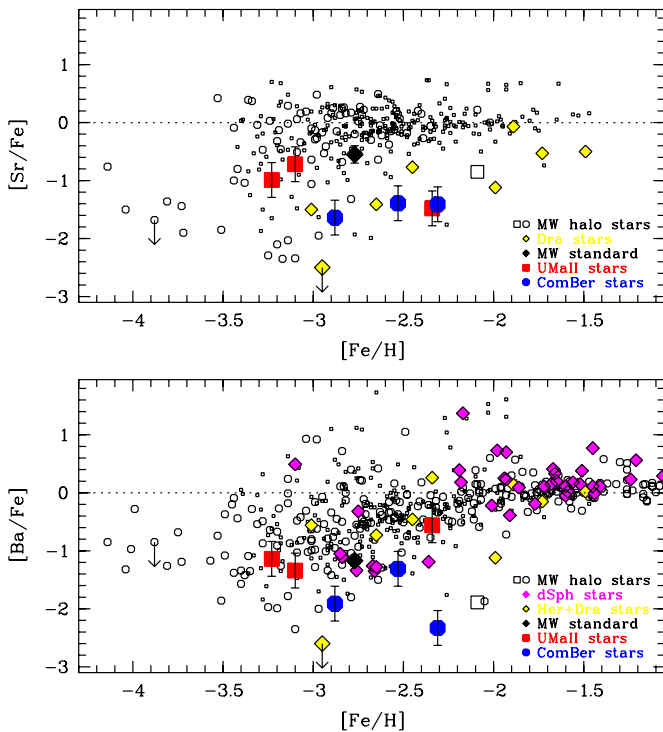
Figure 17. [Sr/Fe] (top panel) and [Ba/Fe] (bottom panel) abundance ratios as a function of [Fe/H]. Except for the upper limit in Dra19 (yellow diamond; Fulbright et al. 2004), these are the first Sr measurements in dwarf galaxies. All the ultra-faint dwarf galaxy [Sr/Fe] and [Ba/Fe] abundances (red squares: UMa II stars; blue circles: ComBer stars) are very low, at the lower end of the distribution of metal-poor halo stars (black squares and circles). Symbols are the same as in Figure 16.
