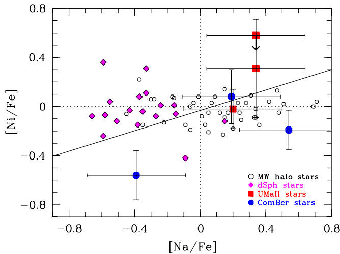
Figure 14. [\text{Ni}/\text{Fe}] ratios for the program stars as function of [\text{Na}/\text{Fe}] in comparison with other objects from the literature (black circles: Cayrel et al. 2004; Lai et al. 2008; pink diamonds: Venn et al. 2004). Blue circles indicate ComBer stars, whereas red squares indicate UMaII stars. The relation found by Nissen & Schuster (1997) is also shown (solid line). The two UMaII stars that deviate most from the Nissen & Schuster relation are also the only two carbon-rich stars in the sample.
