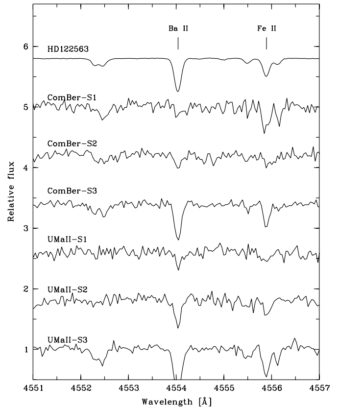
Figure 2. Spectral region around the Ba II line at 4554 Å for the program stars. The Ba and other metallic lines are detected but have significantly different line strengths in each spectrum, confirming the large spread in abundances of these elements in both UMa II and ComBer.
