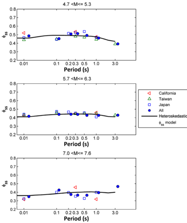
Figure 14. \phi_{ss} values obtained by fitting the magnitude-dependent model to the PEGASOS Refinement Project (PRP) residuals for different magnitude bins ( R \leq 200 km). Results are shown separately for data from three regions, as well as the regions combined. The heteroskedastic \phi_{ss} model is shown for the magnitude corresponding to the center of the magnitude bin. The color version of this figure is available only in the electronic edition.
