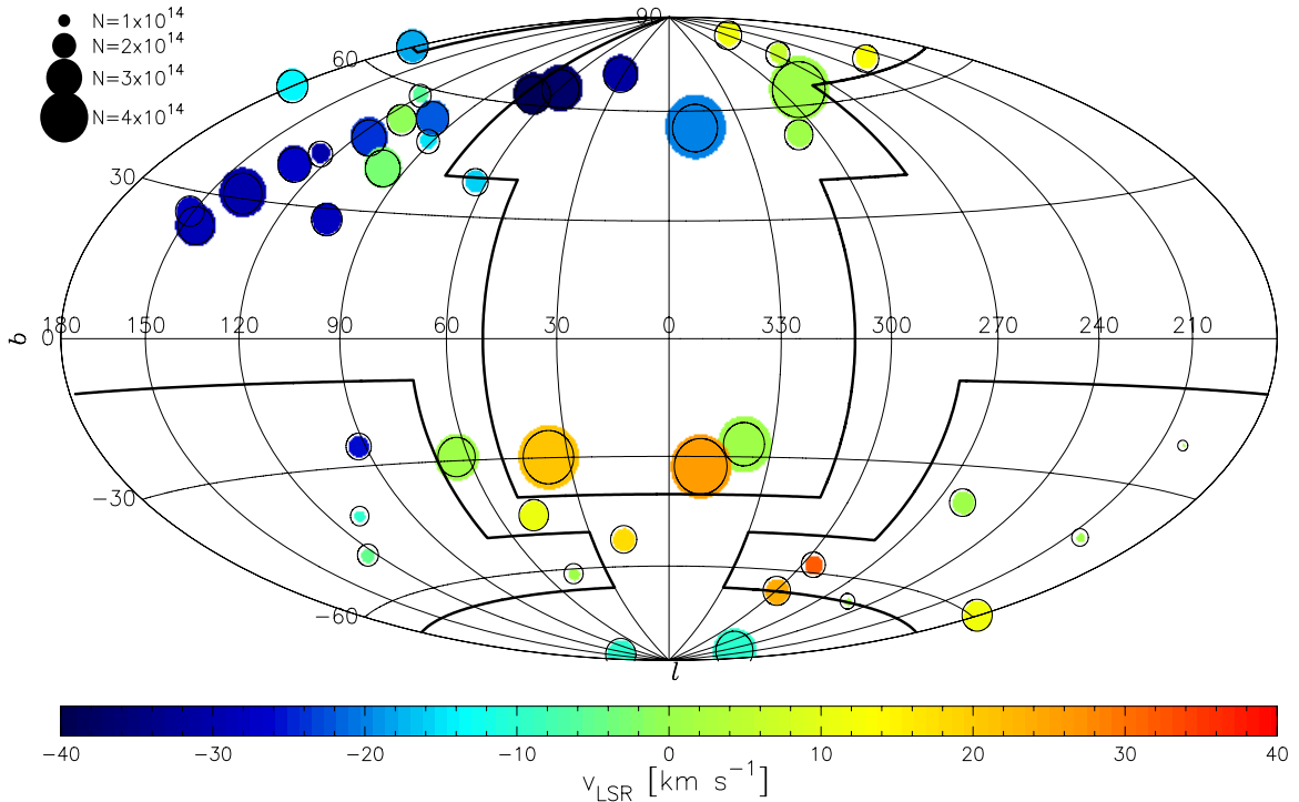
Figure 9. All-sky map of the O VI column density and centroid velocity, in Aitoff projection, centered on the Galactic center. Colors correspond to the centroid velocity of the Galactic O VI absorption, following the scale on the bottom. Symbol diameters are proportional to the value of N(\text{O VI}) , following the legend in the upper left corner. The thick lines outline the regions with an excess or deficit in the O VI column density.
