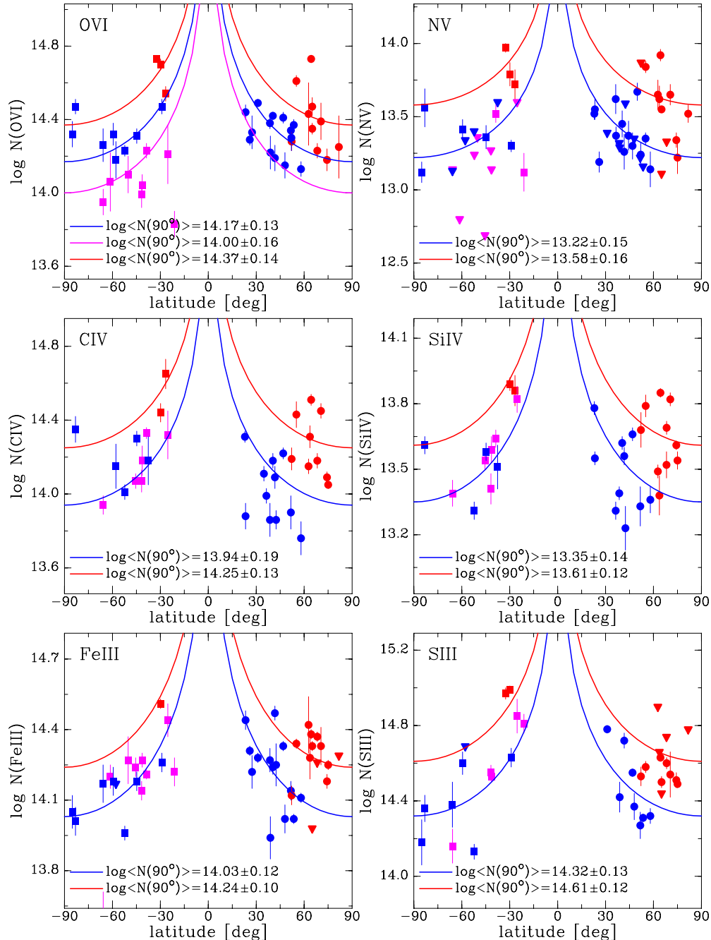
Figure 8. Scatter plot of ionic column densities against Galactic latitude. Symbol types and colors are the same as in Figure 7. In each plot, we also give a curve representing the N(90^\circ) \sin|b| distribution of column densities that would result from a plane-parallel layer, with the values of the corresponding polar column densities given in the lower left corner of each panel.
