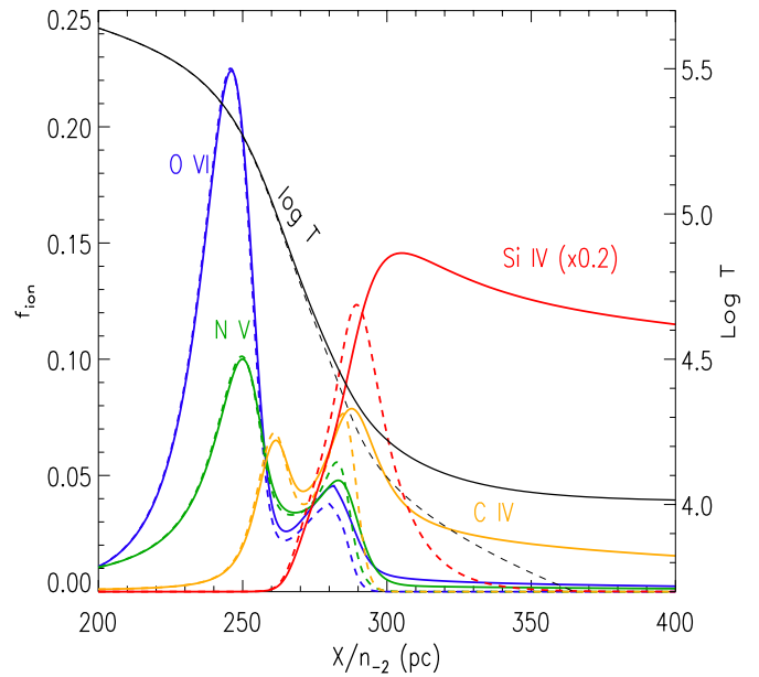
Figure 14. Ionization fractions (left axis) and temperature (right axis) as a function of normalized position for isochorically cooling gas with v_0 = 30 \text{ km s}^{-1} for cases that include (solid) and do not include (dashed) the effects of photoionization. For clarity, the ionization fraction of Si IV has been multiplied by 0.2. The thickness of the zones scales linearly with v_0 , although the zones where C IV and Si IV occur become more extended due to the enhanced photoionization.
