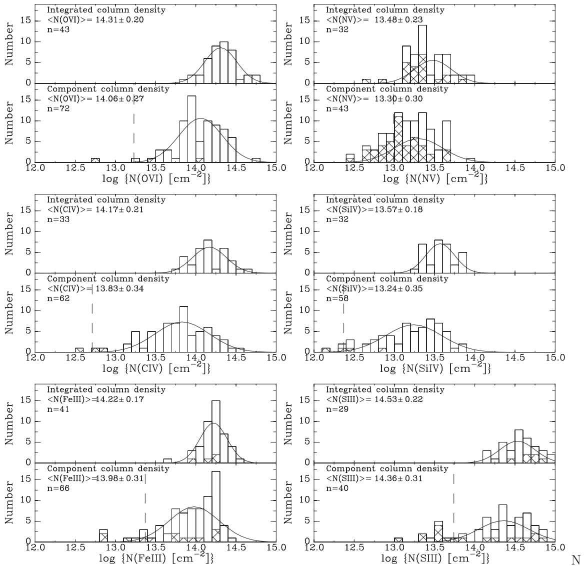
Figure 6. Distributions of column densities for the four high- and two intermediate-ionization species. The top panel of each pair is for the integrated column densities, the bottom panel for the individual components. The hatched parts of the histograms correspond to upper limits. The dotted vertical lines in the bottom panels show the detection limit for a 20 mÅ line with FWHM 40 km s -1 , while the curves are Gaussians using the parameters listed in the label (i.e., number, average, and dispersion). Limits were excluded in these calculations (see the text for a discussion of why this is justified in the case of N v).
