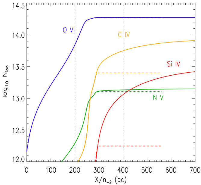
Figure 13. Cumulative column density of highly ionized gas as a function of (normalized) path length through an isochoric radiative cooling flow with v_0 = 30 \text{ km s}^{-1} . The solid and dotted lines show the column density with and without the inclusion of photoionization from the radiation field produced by the cooling gas.
