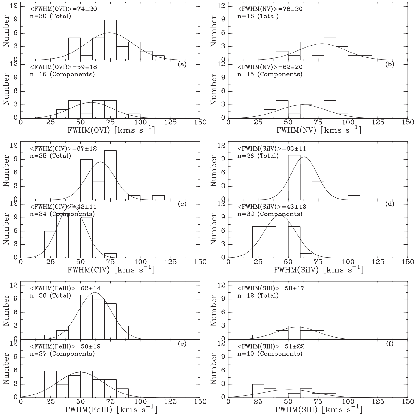
Figure 4. Distribution of line widths for the six ions. There are two panels for each ion, with the top panel in each pair showing the distributions of the FWHM (calculated from the second moment) for the integrated Galactic absorption, and the bottom panel showing the values for individual components. The FWHM of the full Galactic absorption profile is a general indicator for the velocity spread of the high-ionization absorption associated with the Milky Way disk and lower corona. The FWHM of the individual components indicates the velocity spread in single structures. The average and spread of each distribution are given in the label, as are the number of sight lines/components that are used.
