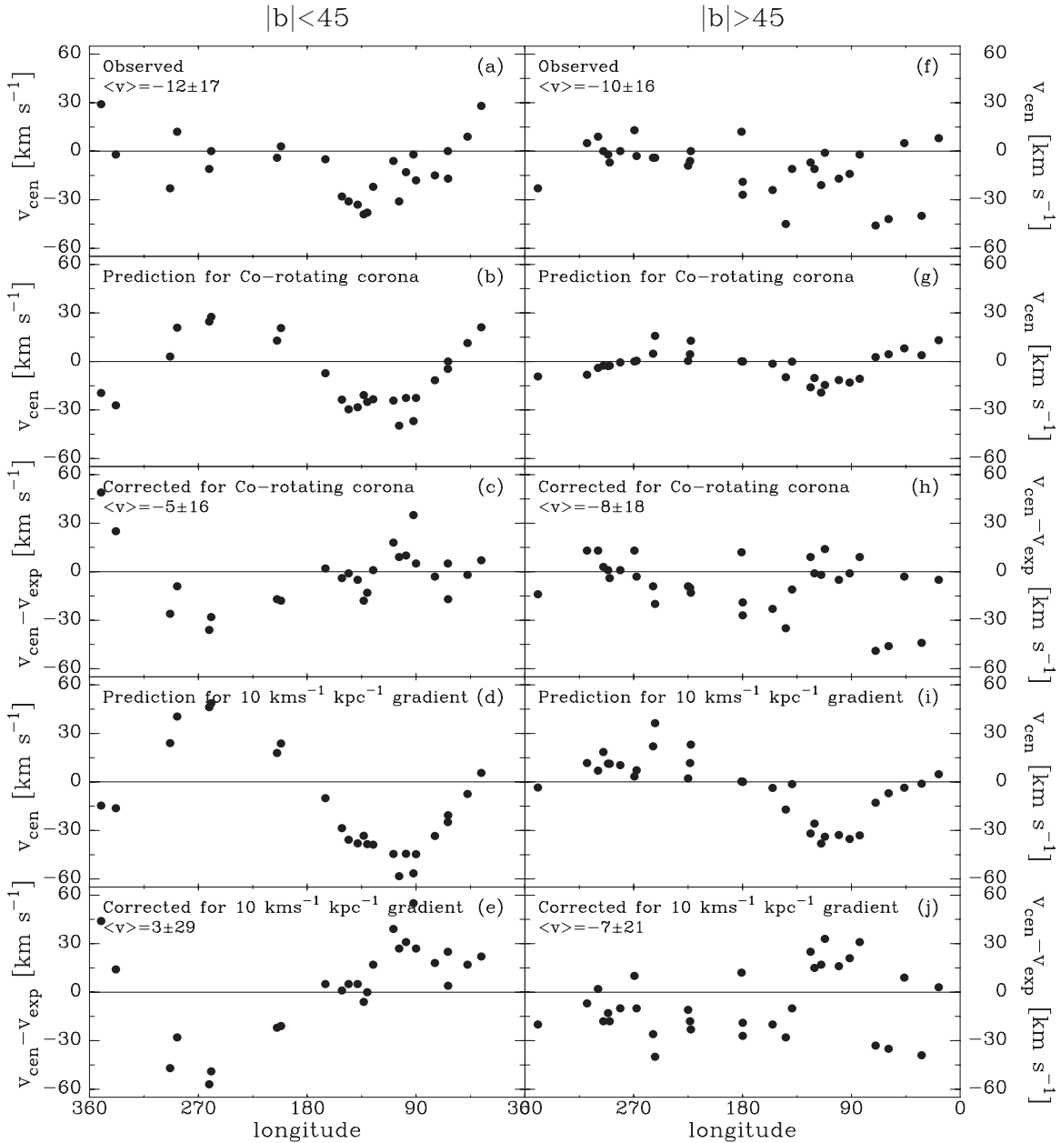
Figure 5. Comparison of observed and expected centroid velocities of the profiles of absorption by highly ionized atoms, as a function of longitude. Panels on the left are for sight lines at low latitudes ( |b| < 45^\circ ), panels on the right are for high latitudes. The top panels give the observations for O VI. The second and third panels give the predictions and difference between observed and predicted values for a corotating corona, while the bottom two panels give this for a corona having a 10 \text{ km s}^{-1} decrease in velocity per kiloparsec away from the Galactic midplane.
