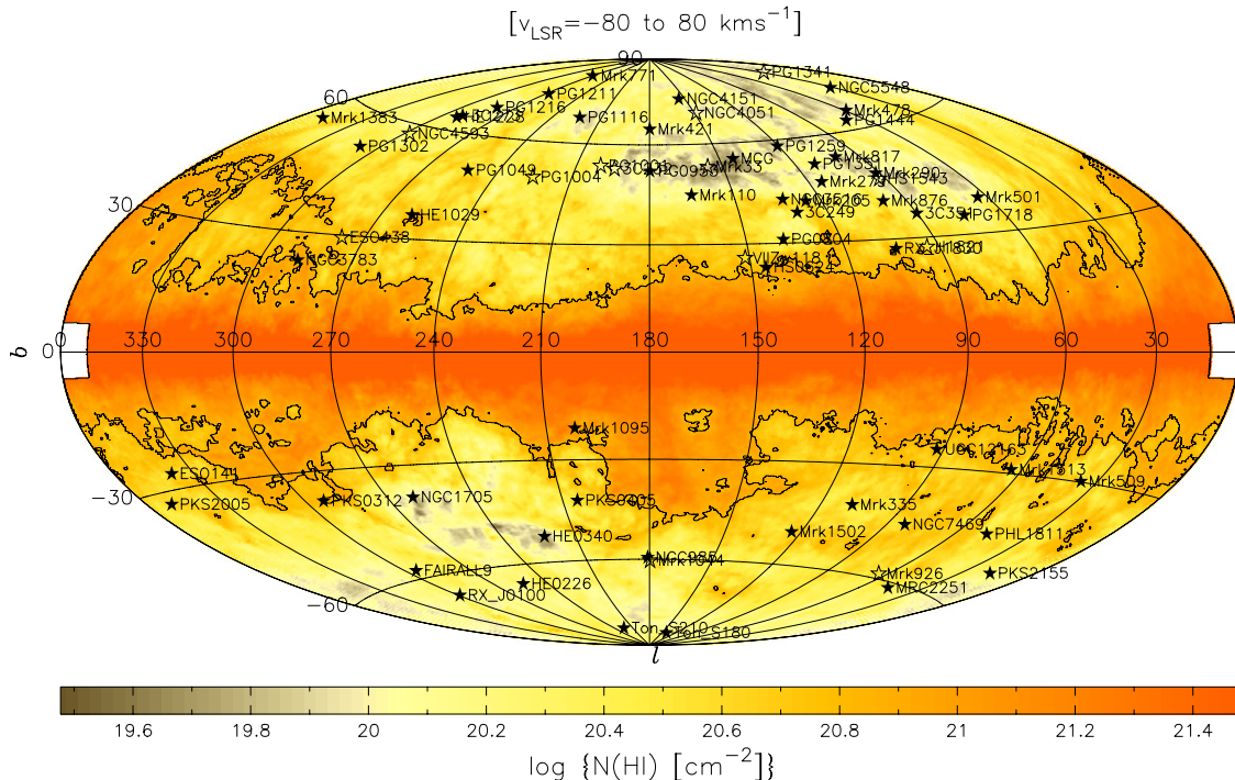
Figure 1. Distribution of targets with N v and/or C IV spectra, on top of a map of the logarithm of the column density of the 21 cm HI sky, integrated between –80 and 80 km s -1 , with a contour overlaid for N(\text{HI}) = 7 \times 10^{20} \text{ cm}^{-2} . The data are shown in an Aitoff projection of Galactic coordinates centered on the anti-center direction. The HI data are from the Leiden–Argentina–Bonn (LAB) survey (Kalberla et al. 2005).
