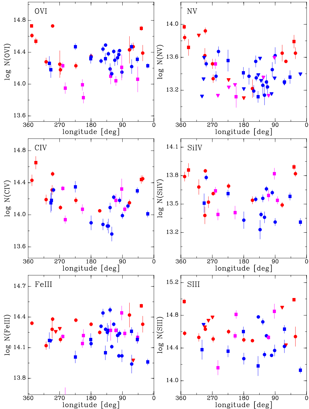
Figure 7. Scatter plot of ionic column densities against Galactic longitude. Circles are for sight lines with b > 0^\circ ; squares are for sight lines with b < 0^\circ . Triangles correspond to upper limits. Red points are for sight lines where N(\text{O VI}) is systematically enhanced (an area of sky delineated as |l| < 40^\circ , |b| < 50^\circ combined with |l| < 80^\circ , b > 40^\circ ). Purple points are for sight lines showing a systematic deficit in N(\text{O VI}) (approximately l = 70^\circ\text{--}280^\circ , b = -60^\circ to -10^\circ ) and blue points cover the rest of the sky.
