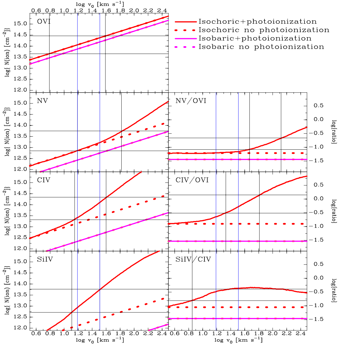
Figure 15. Left panels: column densities as a function of the logarithm of the flow velocity, v_0 , for cases with isobaric cooling (magenta line) and for isochoric cooling with and without photoionization (red solid and red dashed line). Note that the column densities are linearly proportional to flow velocity for low velocities. Note the significant photoionization boost for N v, C iv, and Si iv, setting in at \log v_0 \sim 1.4, 1.0 , and 0.7 , respectively. Right panels: selected column density ratios as a function of the logarithm of the flow velocity. In all panels the observed 1.5\sigma range around the average ionic column density or ratio observed in the Galactic corona is shown with horizontal lines. The averages and dispersions can be found in Sections 4.5 and 4.8. In all panels, vertical lines show the range of velocities, v_0 , for which the predicted column density or ratio falls within the observed range. The solid blue vertical lines show the velocity range within which all four column density predictions fit the observed range ( 15\text{--}32 \text{ km s}^{-1} ).
