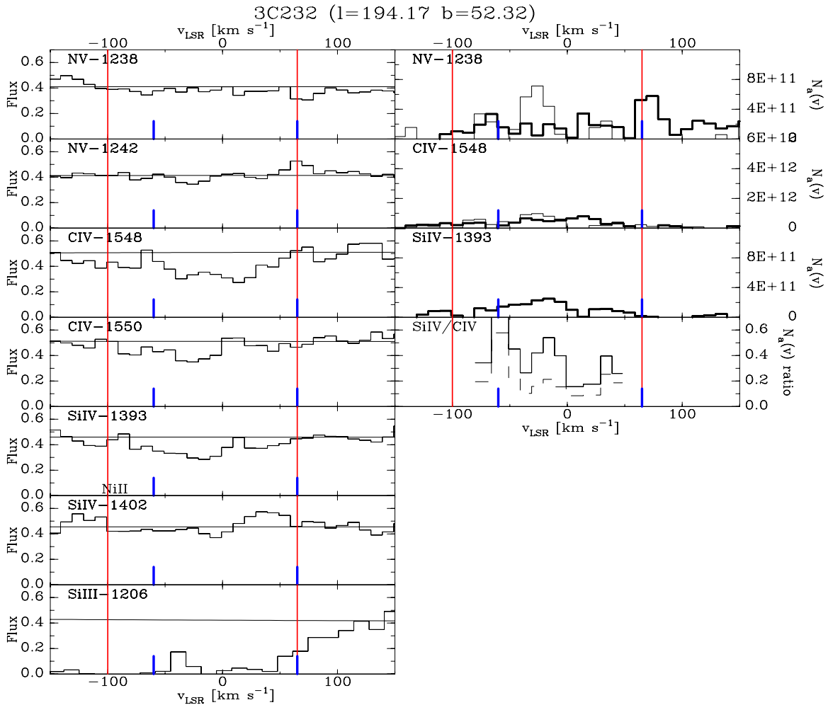
Figure 2. Panels show the available data for the four high-ionization lines, as well as for a strong and a weak intermediate-ionization and a strong and weak low-ionization line (when data are available). The panels on the left give the spectra for the high-ionization lines, as shown by the labels. The top set of panels on the right shows the apparent optical depth profiles for the high-ionization species, with the stronger absorption line shown as thick lines. No apparent optical depth profiles are shown for lines that were deemed unmeasurable, even though a panel is always shown if data were present. Below the optical depth profiles are panels showing the ratios between two ions, but only in spectral regions where the S/N in the ratio is >3 in a 10 \text{ km s}^{-1} velocity bin. Strong intermediate ionization is represented by Si III (or by C III when Si III is not available). Weak intermediate ionization is given by Fe III. The strong low-ionization line is either C II \lambda 1334.532 or C II \lambda 1036.337 , while the weak low-ionization line is S II \lambda 1250.584 or Ar I \lambda 1048.220 . The intermediate- and low-ionization lines are always given in the bottom one or two panels. Line identifications are given at the top left of each panel. The continuum fit (including a model for \text{H}_2 absorption) is also shown. In a few cases (e.g., for O VI \lambda 1037.617 toward Mrk 509), the continuum looks much higher than the data, because it was fit through pixels far outside the displayed range of velocities. All spectra were rebinned to 10 \text{ km s}^{-1} pixels. Other absorption lines in each spectral window are identified by labels near the bottom of each panel. The short vertical blue lines show the range of velocities within 60 \text{ km s}^{-1} of those consistent with standard Galactic differential rotation (see Section 4.2 for the justification of this number). The red vertical lines indicate the velocity limits of integration for the different Galactic components. Note that a figure is available for each sight line in the online version of the journal.
