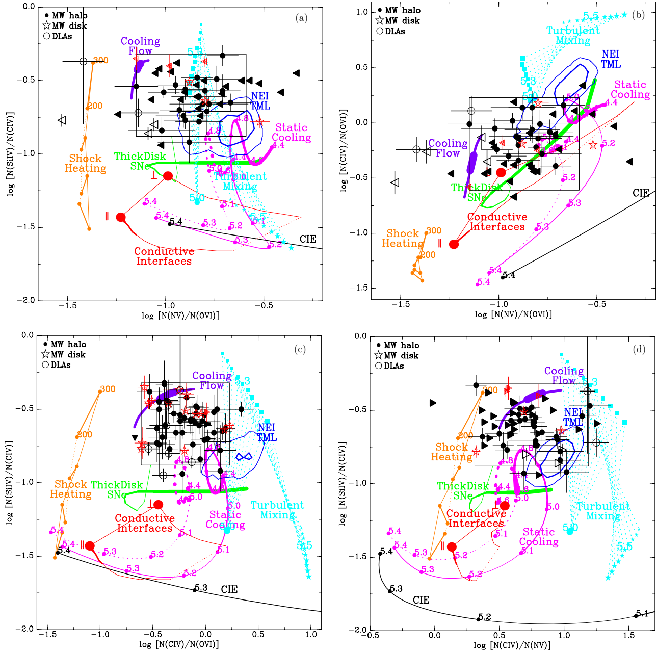
Figure 11. Theoretical ranges and observed values for pairs of ionic ratios. DATA: Filled black circles show ratios in individual components, as determined in Section 3, black triangles show cases with one ratio measured, but the other ratio being an upper or lower limit. A black box outlines the region given by \langle R \rangle \pm \delta R , where the average \langle R \rangle and spread \delta R of the ratio distribution can be found in Figure 10. Open red stars and red triangles represent the results of Lehner et al. (2011), limited to their stars numbered 1, 2, 6, 8, 9, 10, 11, 12, 13, 14, 23, 27, 28, 32, 33, 35, and 38, i.e., not including stars for which the lines are saturated, have very complex component structure, or difficult to determine stellar continua. Note that this selection leaves just six sight lines with measured values for N v, while in two other sight lines O VI is missing; thus fewer than 12 symbols show up in each individual ratio–ratio plot. Open black circles and triangles represent measurements in DLAs at redshifts 2.0–3.1, as presented by Fox et al. (2007). MODELS: (a) Black line (label: CIE): ratios in collisional ionization equilibrium, as calculated by Gnat & Sternberg (2007), for temperatures ranging from \log T = 5.4 to \log T = 4.4 . (b) Magenta lines (label: Static Cooling): non-equilibrium radiative cooling models from Gnat & Sternberg (2007) for temperatures ranging from \log T = 5.4 to \log T = 4.4 , with a solid line for solar metallicity and a dotted line for two times solar metallicity; the line gets thicker at lower temperatures, where the gas spends more time; the gas traverses this trajectory in about 3 \times 10^4/n_0 (cm ^{-3} ) yr. In these models the gas is not flowing, and there is no additional heat input or output. (c) Orange lines (label: Shock Heating): Dopita & Sutherland (1996) shock models, with shock velocities of 200 and 300 km s ^{-1} for the no-magnetic-field case marked and connected by a thick line; the other three thick line segments connect the 200 and 300 km s ^{-1} case for higher magnetic parameters, B n^{-3/2} = 1, 2 and 4 \mu\text{G cm}^{-3/2} . (d) Red lines (label: Conductive Interfaces): the Borkowski et al. (1990) conductive interface predictions; a “perpendicular” and a “parallel” symbol mark which of the two lines is for perpendicular or parallel magnetic field; the line thickness increases linearly with the age of the interface, 0.1 Myr at the thinnest point, 10 Myr at the other end, which is reached after 1–2 Myr. As a result, the line for this model appears as a quickly traversed thin red line ending in a large dot, where the ratios stabilize. (e) Green line (label: thick disk SN): the Shelton (1998) thick disk supernova model (SNe occurring at heights up to 2 kpc), giving the evolution of the ratios with time (from 1 to 16 Myr in age), with the line thickness proportional to the amount of time spent at each point. (f) Light blue lines (label: Turbulent Mixing): predictions of the Slavin et al. (1993) semi-analytic turbulent mixing layer model; circles, squares, and stars are shown for entrainment velocities ranging from 25 to 100 km s ^{-1} at temperatures of \log T = 5.0, 5.3 , and 5.5 , respectively; the symbol size is proportional to the entrainment velocity. (g) Solid blue contours (label: NEI TML): distribution of ratios in the Kwak & Shelton (2010) turbulent mixing layer models, corresponding to 256 column densities derived by integrating through an interface at 1 Myr intervals for ages between 20 Myr and 80 Myr. (h) Dark purple line (label: Cooling Flow): the predictions of the model by Benjamin & Shapiro that is described in the Appendix. This model is applicable to cooling hot gas flowing through an interface. The range of flow velocities is 20–30 km s ^{-1} (thicker part of the line) and 12–42 km s ^{-1} (thinner part). For these flow velocities the absolute column densities are within 2 and 1 times the observed dispersion around the observed average value.
