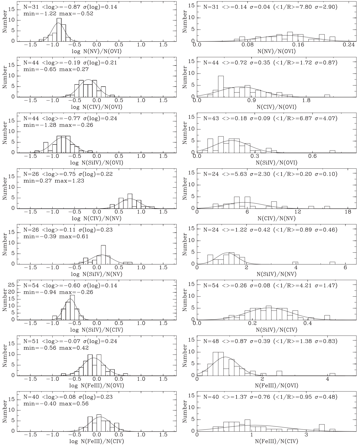
Figure 10. Histograms of the distribution of the logarithmic (left panels) and linear ratios (right panels) between O VI, N v, C IV, Si IV, and Fe III. The number of measurements ( N ), average ( \langle \log \rangle ), and dispersion ( \sigma(\log) ) of each ratio distribution are given in the top left corner. The second line gives the range of values. Gaussians with the listed parameters are overlaid. To make comparisons with other papers easier, in the panels on the right, the average linear ratio and its dispersion are given, as are the average and dispersion of the distribution of the inverse ratio. For example, the average ratio of N v/O VI is 0.14, while the average ratio of O VI/N v is 7.80.
