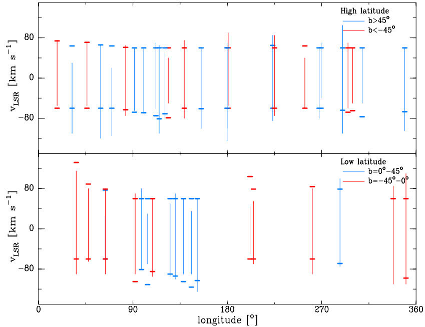
Figure 3. Comparison of the extent of the Galactic high-ionization absorption with the range of velocities allowed by differential galactic rotation, as function of galactic longitude. The thick horizontal bars are placed at velocities \pm 60 \text{km s}^{-1} larger/smaller than the maximum/minimum velocity expected from rotation. The vertical lines indicate the observed range of velocities over which high-ionization absorption is seen. The top panel shows high-latitude sight lines and the bottom panel shows low-latitude sight lines, with northern sight lines in blue and southern sight lines in red.
