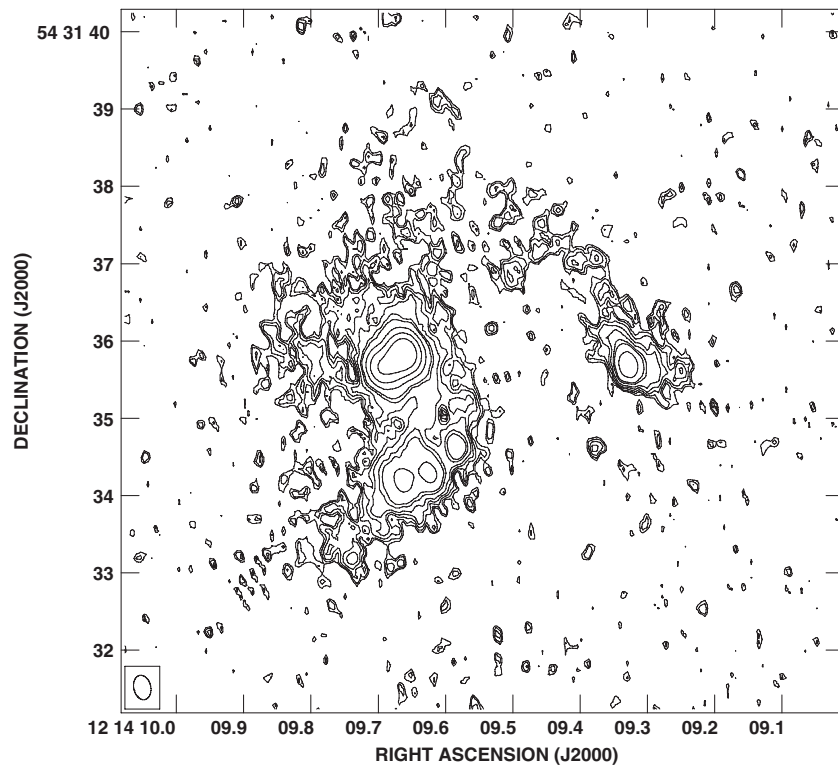
Figure 3. Low-level emission at 3.6 cm. The 0''.32 \times 0''.22 beam is shown. The lowest contour is 1.3\sigma ( 0.02 \text{ mJy } \text{bm}^{-1} ) and contour levels are 1, 1.4, 2, 2.8, 4, 6.25, 8, 16, 32, and 64.
