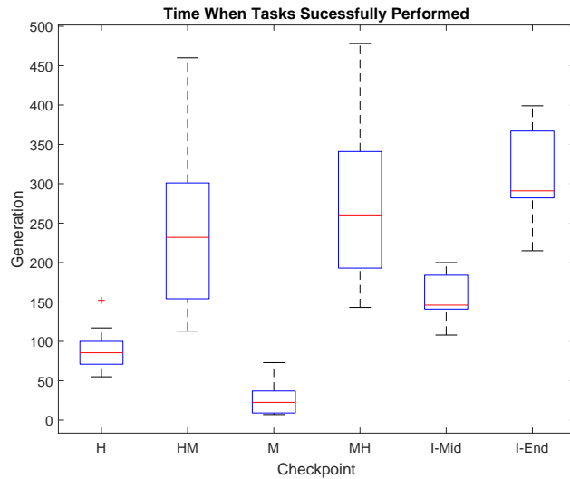
Figure 4: Boxplots showing how long it takes to achieve task success in the three experiments. From left to right, H is the population after only evolving hunting, HM after evolving hunting and then both, M after mating only, and MH after mating then both. I indicates that the two tasks were interleaved, and the population in this experiment is analyzed at both the mid- and end-point of the evolutionary run. Evaluated alone, the mating task evolved before the hunting task, while both took less time than the interleaved tasks. But the difference between mating and hunting disappears after the second task is introduced.
