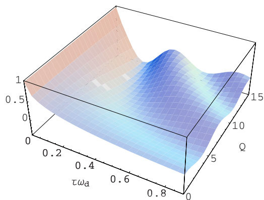
FIG. 3. (Color online) The surface plot of normalized autocorrelation function C(\tau)/\sigma^2 as a function of normalized time differences \tau\omega_d and the quality factor Q .
