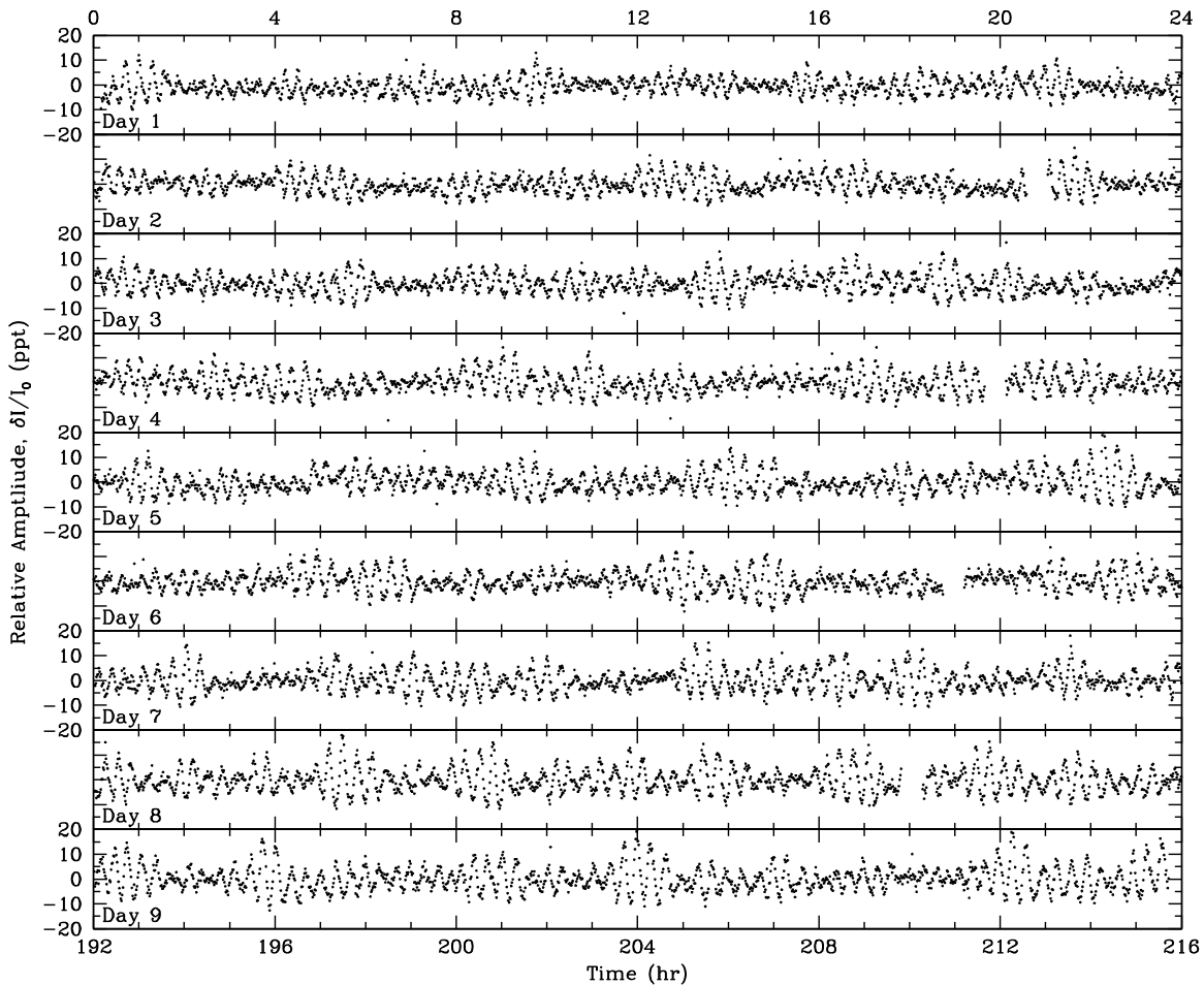
Figure 1. Portion of the minute-cadence photometry collected on the pulsating white dwarf GD 1212 in 2014 February. This 9.0 day light curve (shown without any smoothing) establishes the capabilities of a two-wheel-controlled Kepler spacecraft on this K_p = 13.3 mag white dwarf. An additional 2.6 days of data, not shown, were collected on GD 1212 in 2014 January and included in our analysis.
