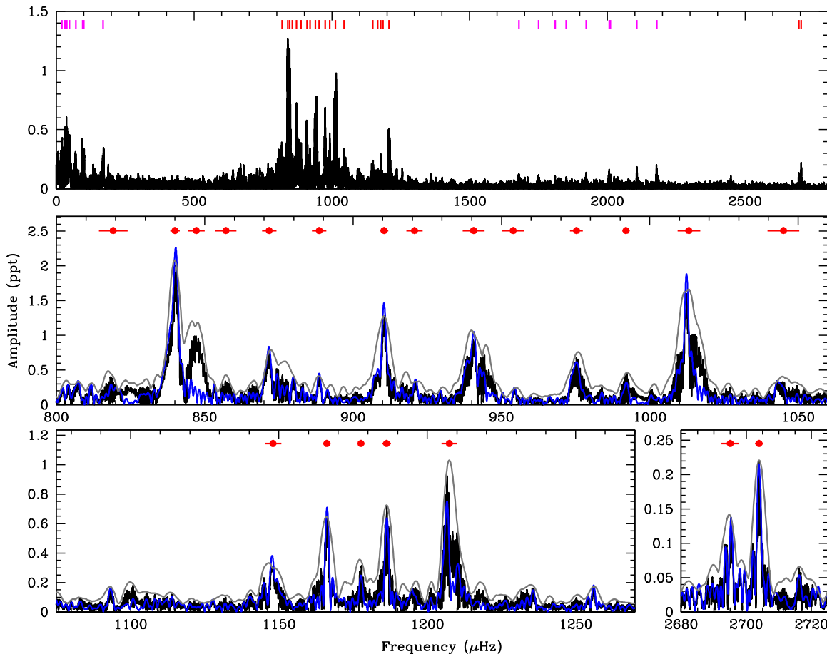
Figure 2. Fourier transforms (FTs) of our two-wheel-controlled Kepler observations of GD 1212. The top panel shows the FT of the entire data set out to 2800 \mu\text{Hz} ; there are no significant periodicities at longer frequencies. The middle and bottom panels show the independent pulsation modes in more detail. The blue FT represents only the final 9.0 days of data, while the black FT was calculated from the entire 26.7 day data set. Additionally, we have split the data into four 2.6 day subsets, and we average the amplitudes of the FTs of each of these subsets, shown in gray for the bottom two panels. We mark the pulsation modes adopted, detailed in Table 1, with red points and associated uncertainties at the top of each panel. Additionally, the magenta lines in the top panel mark nonlinear combination frequencies also detected in our data, shown in more detail in Figure 4. Amplitudes are expressed in ppt, where 1 ppt = 0.1% relative amplitude.
