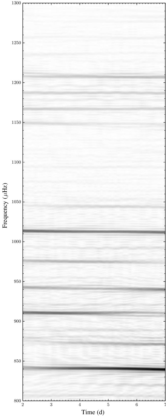
Figure 3. Running FT of the range of independent pulsation modes detected in our 9.0 day, high-duty-cycle two-wheel-controlled Kepler light curve of GD 1212. This figure uses a four-day sliding window, and darker grayscale corresponds to higher amplitudes. This demonstrates the lack of amplitude and frequency stability for the pulsations in GD 1212, even over less than a week.
