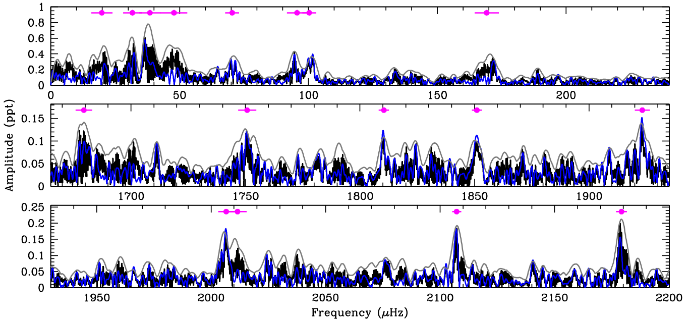
Figure 4. Fourier transforms (FTs) of the nonlinear combination frequencies detected in our observations of GD 1212. As in Figure 2, the blue FT represents only the final 9.0 days of data, while the black FT was calculated from the entire 11.6 days of data spread over 26.7 days. Additionally, the average FT of four 2.6 day subsets is shown in gray. We mark the adopted combination frequencies, detailed in Table 1, with magenta points and associated uncertainties at the top of each panel.
