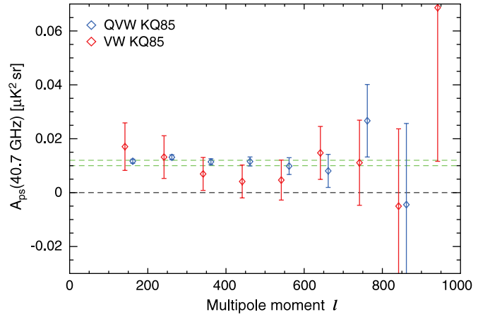
Figure 3. Unresolved point source contamination A_{\text{ps}} , measured in bins of \Delta\ell = 100 evaluated at 40.7 GHz (Q band). For a source population whose fluxes are independent of frequency A_{\text{ps}} scales roughly as \sim \nu^{-2} in the WMAP data. The red data points are from the analysis of V and W bands alone and the blue points are from the analysis of Q, V, and W bands. The horizontal dashed green lines, at 0.010 and 0.012, show the 1\sigma bounds for our adopted value of A_{\text{ps}} . Note that the QVW amplitude is independent of \ell .
