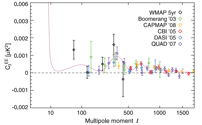
Figure 10. WMAP five-year EE power spectrum, compared with results from the Boomerang (Montroy et al. 2006, green), CAPMAP (Bischoff et al. 2008, orange), CBI (Sievers et al. 2007, red), DASI (Leitch et al. 2005, blue), and QUAD (Ade et al. 2008, purple) experiments. The pink curve is the best-fit theory spectrum from the \Lambda CDM/ WMAP Markov chain (Dunkley et al. 2009). Note that the y-axis is C_l^{\text{EE}} , not l(l+1)C_l^{\text{EE}}/(2\pi) .
