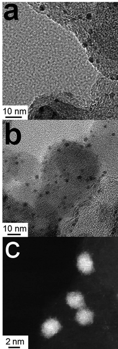
Fig. 4 TEM micrographs of Au 147 @Pt 102 DENs (a) before and (b and c) after being used for the ORR. The particle diameters before and after the ORR were 2.3 ± 0.4 and 2.4 ± 0.4 nm, respectively.
