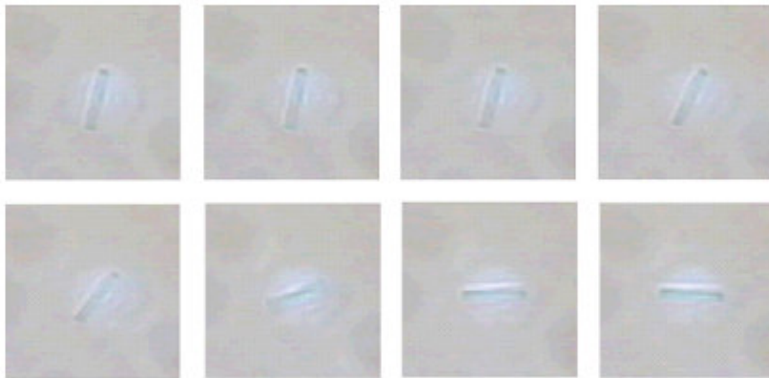
Figure 3. Microscopic glass cylinders following the rotating plane of polarization of the trapping beam. The length of the cylinder is 1.8 \mu\text{m} . Source: Bishop et al. (2003).
