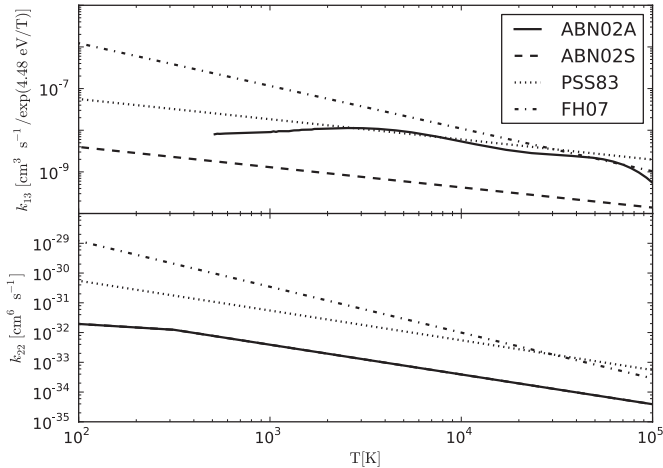
Figure 1. Collisional dissociation (top) and three-body association (bottom) rates from ABNO2 (solid: simulation ABNO2A, dashed: ABNO2S), PSS83 (dotted: simulations PSS83A and PSS83S), and FH07 (dash-dot: simulations FH07A and FH07S). A factor of \exp(4.48 \text{ eV}/T) has been divided out of the collisional dissociation rate for clarity. We note that the solid and dashed lines, for simulations ABNO2A and ABNO2S, are coincident in the lower panel.
