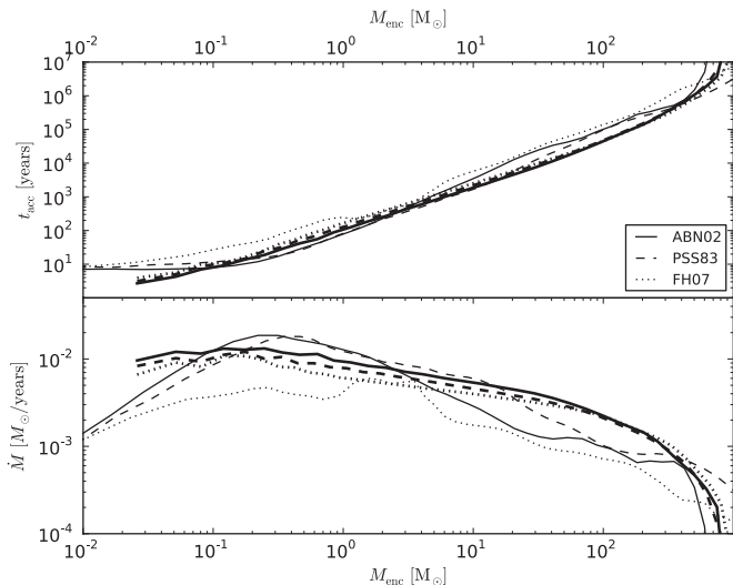
Figure 7. Radially binned, spherically averaged accretion times (top) as a function of enclosed mass and the accretion rates (bottom) for each mass shell. These values were calculated at the final output time of the simulation. Thin lines correspond to the AMR simulations and thick lines correspond to the SPH simulations.
