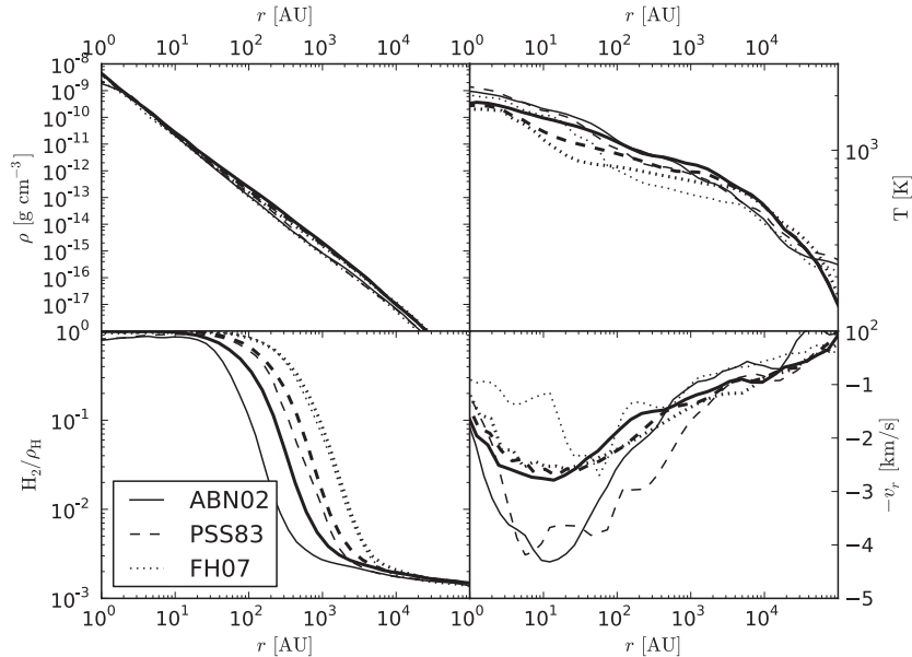
Figure 4. Radially binned, spherically averaged profiles of density (volume-weighted, upper left), temperature (mass-weighted, upper right), molecular hydrogen mass fraction (mass-weighted, lower left), and radial velocity (mass-weighted, lower right) plotted as a function of radius from the most dense point in the calculation. Thin lines correspond to the AMR simulations and thick lines correspond to the SPH simulations.
