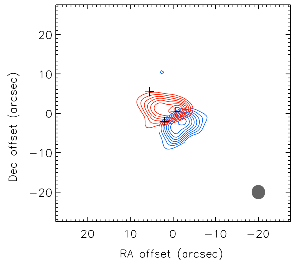
Figure 19. Integrated intensities of blue- and redshifted emission of CO 2-1. Blue contours represent the intensities integrated over the blueshifted range from -20 to -7 \text{ km s}^{-1} and red contours show the intensities integrated over the redshifted range from -2 to 10 \text{ km s}^{-1} . The contours range from 4\sigma of the peak intensity to 90% and increase in steps of 10%. VLA 6, VLA 7, and VLA 10 are denoted by crosses. The beam FWHM is represented by the gray filled ellipse.
