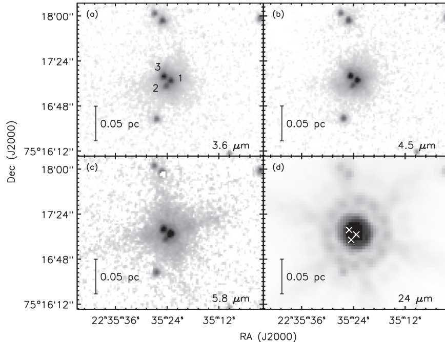
Figure 1. Spitzer images of L1251A in the log scale at (a) IRAC 3.6 \mu\text{m} , (b) IRAC 4.5 \mu\text{m} , (c) IRAC 5.8 \mu\text{m} , and (d) MIPS 24 \mu\text{m} . In Figure 1(d), the Xs indicate the positions of the IR sources in L1251A.
