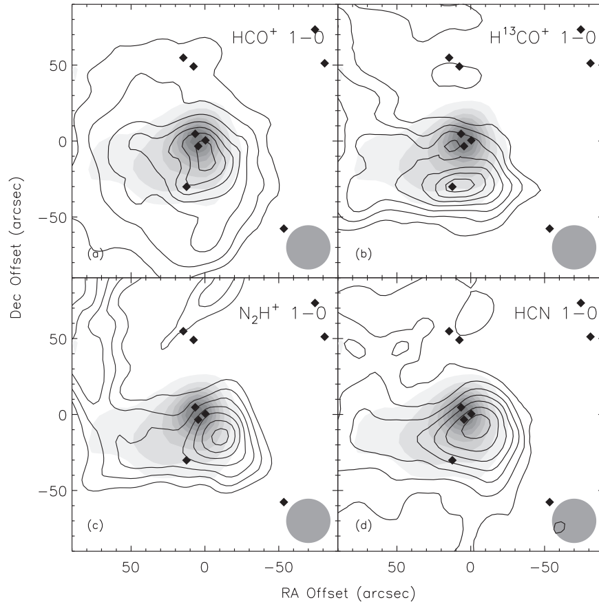
Figure 4. Integrated intensity maps of (a) \text{HCO}^+ 1-0 , (b) \text{H}^{13}\text{CO}^+ 1-0 , (c) \text{N}_2\text{H}^+ 1-0 , and (d) \text{HCN } 1-0 on top of the 850\ \mu\text{m} map (gray scale). Contour intervals are 10% of the each peak intensity and range from 35 to 95%. The gray scale levels are 20, 40, 60, 80, and 100% of the peak intensity, 1.20\ \text{Jy beam}^{-1} . YSO candidates are denoted by filled diamonds. The filled circle at the bottom right of each panel denotes the respective beam FWHM.
