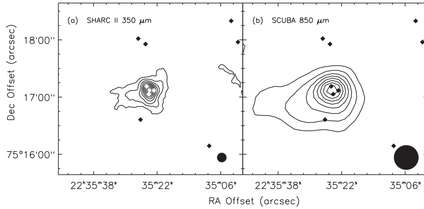
Figure 3. Dust continuum emission map toward L1251A. (a) Continuum emission at 350\ \mu\text{m} obtained with SHARC-II at the CSO (Wu et al. 2007). Contour levels are 20, 40, 60, 80, and 100% of the peak intensity, 5.40\ \text{Jy beam}^{-1} . (b) Continuum emission at 850\ \mu\text{m} obtained with SCUBA at the JCMT (Di Francesco et al. 2008). Contour levels are 20, 40, 60, 80, and 100% of the peak intensity, 1.20\ \text{Jy beam}^{-1} . The respective beam FWHM is presented in each panner with filled circle. YSO candidates are denoted by filled diamonds.
