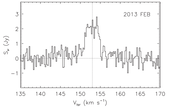
Figure 8. Highest velocity component of 22 GHz \text{H}_2\text{O} maser line toward L1251A. This high-velocity component was detected only on 2013 February. The horizontal dotted line and the vertical dotted line represent the zero baseline and the central velocity of the highest-velocity component, respectively.
