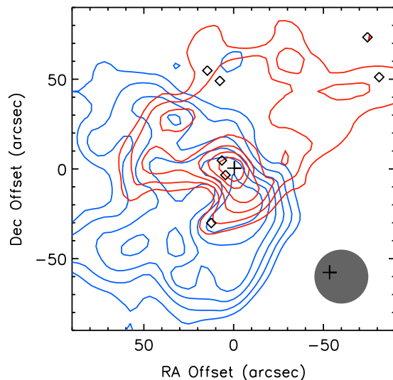
Figure 18. Integrated intensities of blue- and redshifted emission of \text{HCO}^+ 1-0 . Blue contours represent intensities integrated over the blueshifted range from systemic velocity. Red contours show intensities integrated over the redshifted range. The velocity ranges used for the blue and red components are from -9.7 to -5.9 \text{ km s}^{-1} and from -4.0 to -0.2 \text{ km s}^{-1} , respectively. The contours range from 40% of the peak intensity to 90% and increase in steps of 10%. IRS 1 and the other YSOs are denoted by a cross and diamonds, respectively. The beam FWHM is represented by the gray filled circle.
