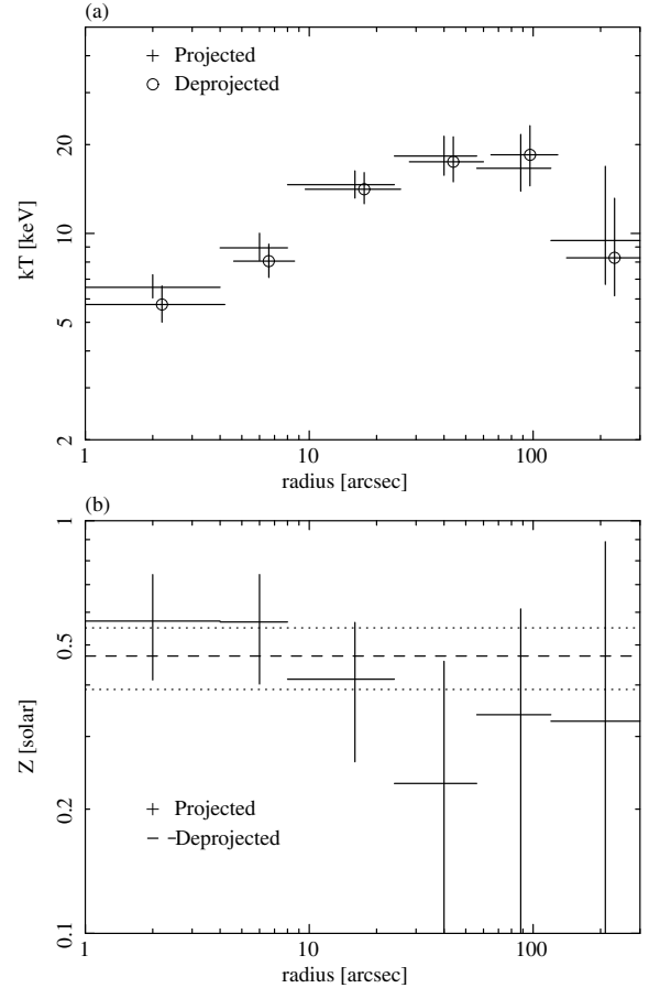
Fig. 10. a) Projected (crosses) and deprojected (circles) temperature profiles measured from the Chandra data in the NW region. b) Projected metal abundance profile (crosses). The horizontal dashed and dotted lines show the best-fit constant abundance and the corresponding 90% confidence interval obtained from the deprojection analysis, respectively. We assume that the metal abundance is constant over all radial bins throughout this paper.
