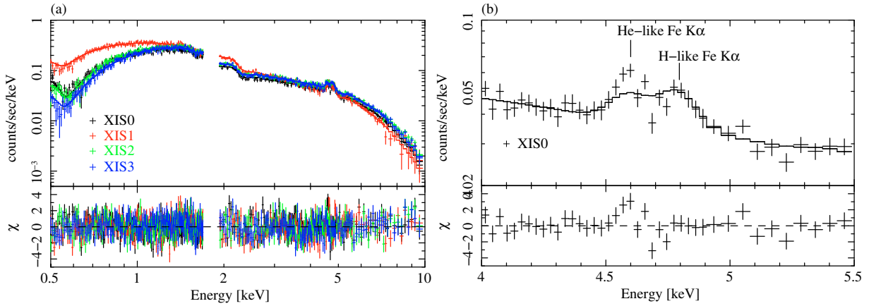
Fig. 2. a) Observed XIS spectra ( r < 5' ). The spectra taken by four sensors, XIS-0 (black), 1 (red), 2 (green), and 3 (blue), are shown separately. The solid lines in the upper panel show the best-fitting single-temperature APEC thermal plasma model simultaneously fit to all of the sensors, convolved with the telescope and the detector response functions. In the bottom panel the residuals of the fit in units of the number of standard deviations are shown. b) Blow-up of the XIS-0 spectrum in the 4–5.5 keV band. The single-temperature kT model fails to fit the He-like Fe K\alpha line.
