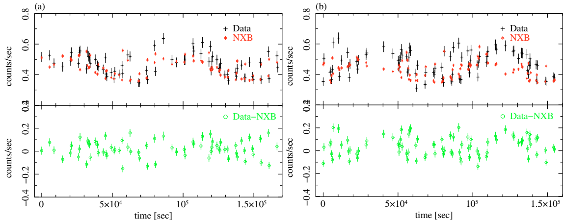
Fig. 6. Observed light curves of the PIN 12–40 keV count rates during two observing periods. a) Seq: 801013010; and b) Seq: 801013020. In the upper panels, the Data and NXB rates are shown by black and red crosses, respectively. In the bottom panels, (Data–NXB) is shown by the green circles. The error bars show the 1\sigma statistical errors.
