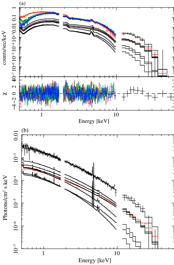
Fig. 11. a ) 6APEC×PLABS ( \alpha = 0.02 ) + APEC model, fit simultaneously to the observed XIS (0.5–10 keV) and PIN (12–60 keV) spectra. The spectra taken by four sensors, XIS-0 (black), 1 (red), 2 (green), and 3 (blue), are shown separately. The black and red lines show the ambient component (6APEC × PLABS) and the excess hot component described by an additional APEC model, respectively, convolved with the telescope and the detector response functions. In the bottom panel the residuals of the fit in units of the number of standard deviations are shown. We have used the nominal NXB model for the background of the PIN data (see Sect. 4.1). b ) same as a ), but for the unfolded XIS-0 and PIN spectra.
