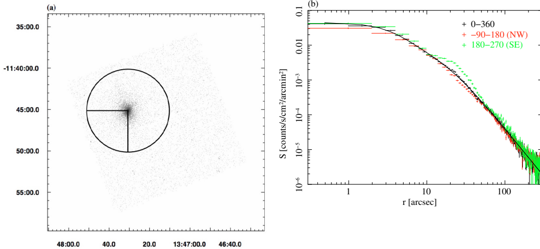
Fig. 9. a) Chandra ACIS-I image in the 0.5–7 keV band. The solid lines show the NW and SE regions. The radius of the circle is 5'. b) The surface brightness profiles of the position angle 0°–360° (black), NW: –90°–180° (red), and SE:180°–270° (green). The black line shows the best-fit double \beta -model for the position angle of 0°–360°.
