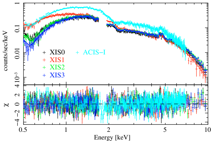
Fig. A.1. Suzaku /XIS+ Chandra /ACIS-I spectra of RX J1347.5–1145 ( r < 5' ) simultaneously fitted with the APEC×PLABS model.
