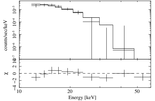
Fig. 8. Observed PIN spectrum with the background model subtracted (Data–NXB–CXB; the crosses) in the 12–60 keV band. The error bars indicate only the statistical errors. The histogram shows the best-fit APEC thermal plasma model. The bottom panel shows the residuals in units of the number of standard deviations.
