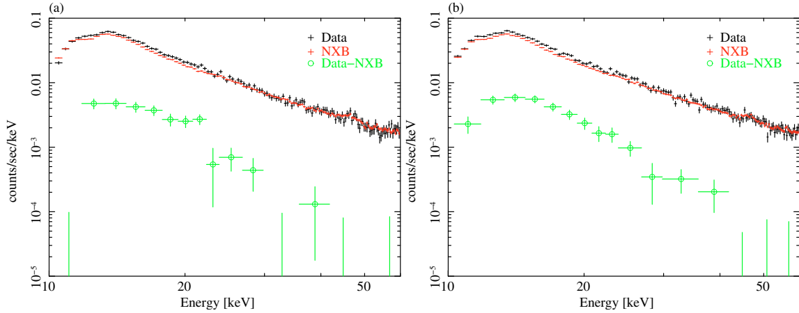
Fig. 5. Observed PIN spectra during two observing periods of RX J1347.5–1145. a) Seq: 801013010; and b) Seq: 801013020. In each panel Data, NXB, and (Data–NXB) are shown with the black crosses, red crosses, and green circles, respectively.
