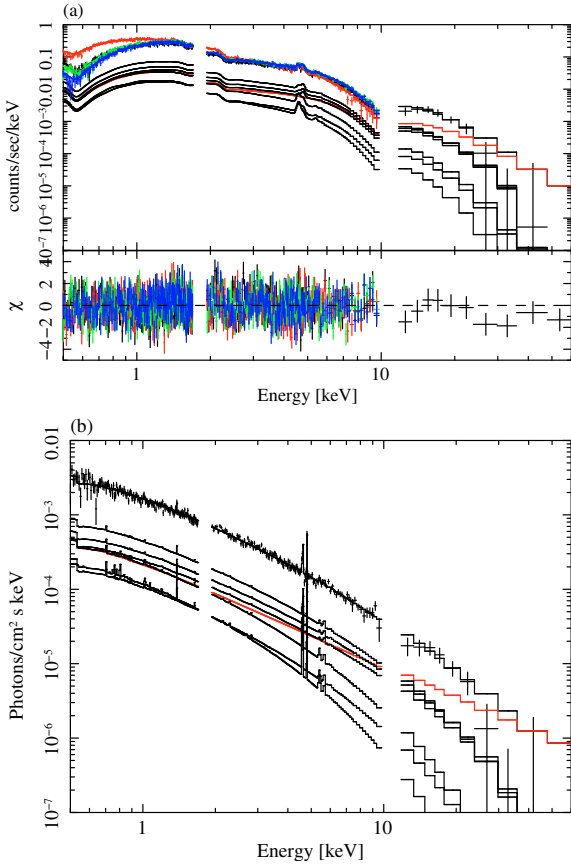
Fig. 12. a) 6APEC \times PLABS ( \alpha = 0.02 ) (thermal model for the ambient gas) + PL model (non-thermal model for the hot gas), fit simultaneously to the observed XIS (0.5–10 keV) and PIN (12–60 keV) spectra. The spectra taken by four sensors, XIS-0 (black), 1 (red), 2 (green), and 3 (blue), are shown separately. The black and red lines show the ambient component (6APEC \times PLABS) and the excess hot component described by a non-thermal power-law model, respectively, convolved with the telescope and the detector response functions. In the bottom panel the residuals of the fit in units of the number of standard deviations are shown. We have used the nominal NXB model for the background of the PIN data (see Sect. 4.1). b) same as a) , but for the unfolded XIS-0 and PIN spectra.
