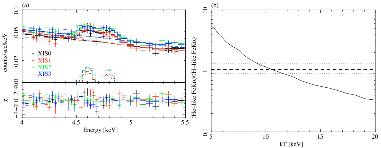
Fig. 3. a) Observed XIS spectra in the 4–5.5 keV band. The spectra taken by four sensors, XIS-0 (black), 1 (red), 2 (green), and 3 (blue), are shown separately. The solid lines in the upper panels are the best-fitting continuum plus two Gaussian models. In the bottom panel the residuals of the fit in units of the number of standard deviations are shown. b) Line ratio (He-like Fe K\alpha )/(H-like Fe K\alpha ) as a function of temperature, calculated from the APEC model. The horizontal dashed line and the dotted lines show the best-fitting line ratio and the 90% confidence interval, respectively.
