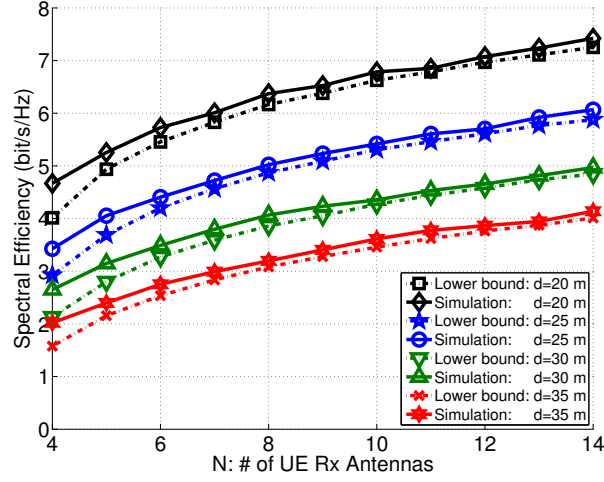
Figure 4.4: Simulated D2D spectral efficiency vs. analytical lower bound (4.22) with perfect CSI and (n_c, n_d) = (0, 2) .
