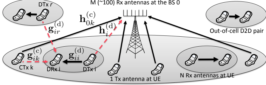
Figure 4.1: A D2D underlaid massive MIMO system consisting of both cellular and D2D links. For clarity, only the central cell is shown. D2D pairs located outside of the cells are out of cellular coverage but still contribute to the total aggregate D2D interference.
