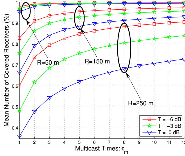
Figure 2.3: Normalized mean number of covered receivers versus multicast times without network assistance.
