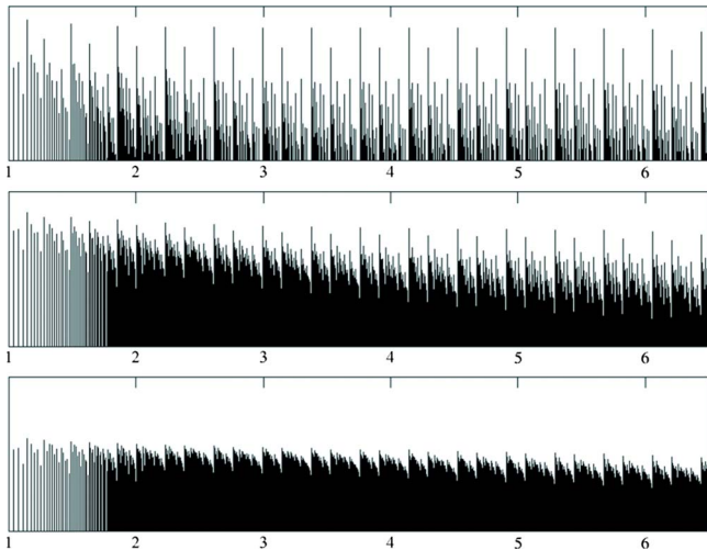
FIG. 7. (Color online) Plot of \log_{10}|k(\widehat{\text{Re } \chi})_k| vs \log_{10}|k| for the maps f_{d,(2^\infty),1+3i} with d=1,5,20 .
