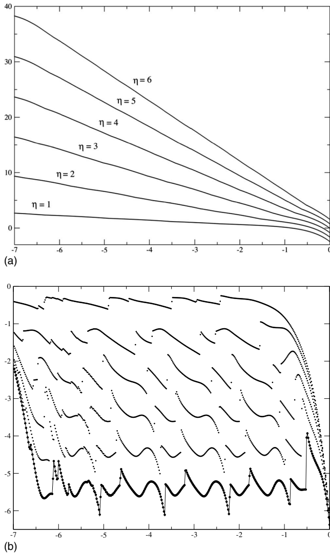
FIG. 9. (Top) plot of \log_{10} N_\eta(\tau) vs \log_{10} \tau for the map (3) with \sigma=(5^\infty) . (Bottom) plot of the differences between the vertical coordinates of adjacent points in the top figure.
