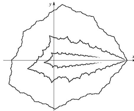
FIG. 2. Siegel disks of the maps f_{d,\langle 2^\infty \rangle, 1+3i} [given by Eq. (4)] with critical point c = 1 of order d = 1 (outermost curve), d = 5 , and d = 20 (innermost curve). See text for details.
