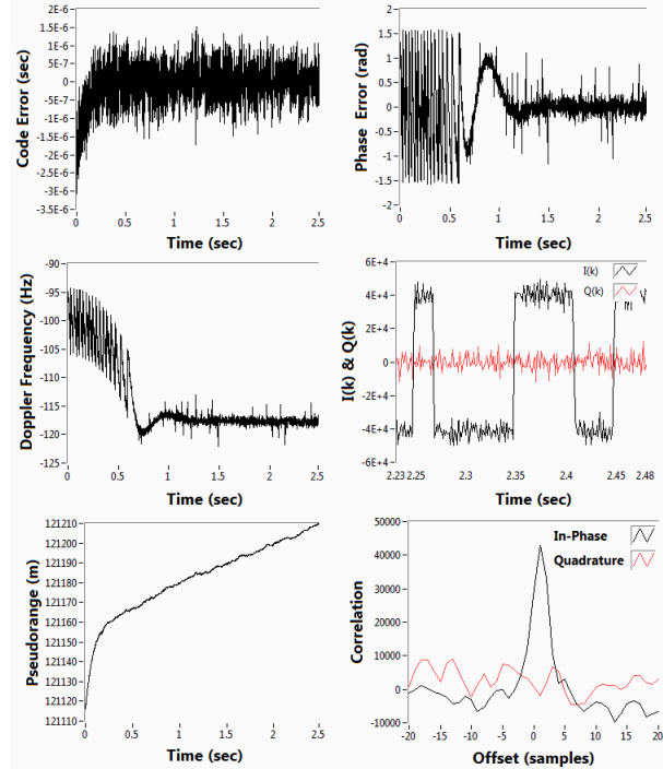
Fig. 5. Front panel of tracking mode
