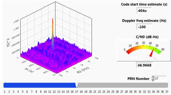
Fig. 4. Front panel of acquisition mode
