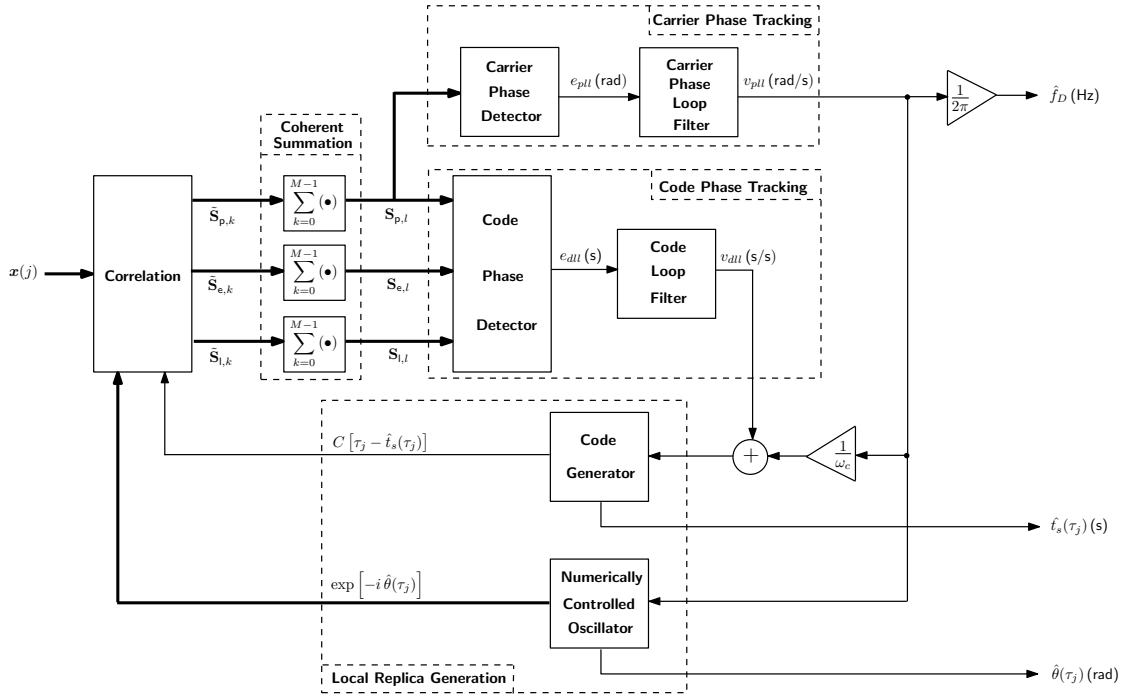
Fig. 1. Block diagram of a single-channel GPS signal tracking. Thick lines indicate complex values.
