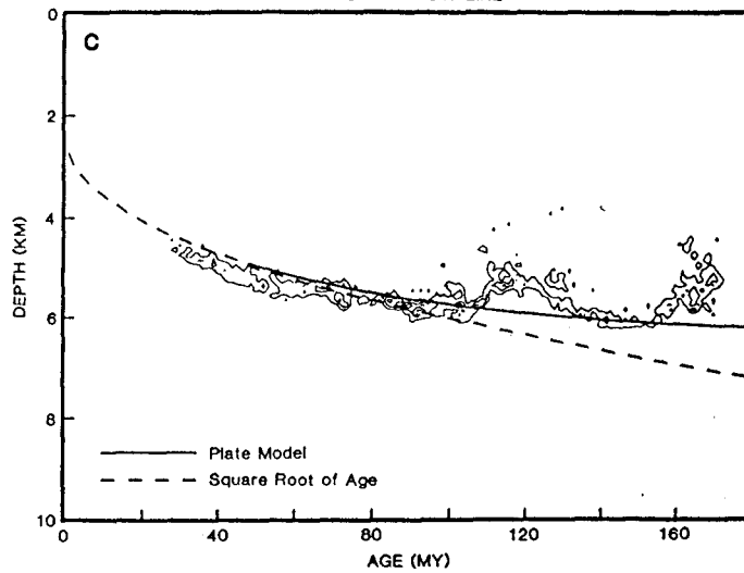
MODE - FLOW LINE
