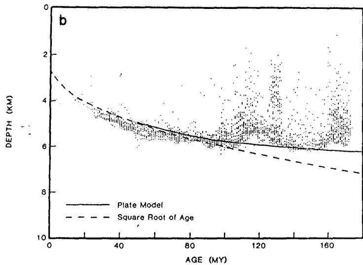
DEPTH VERSUS AGE ALONG FLOW LINE
