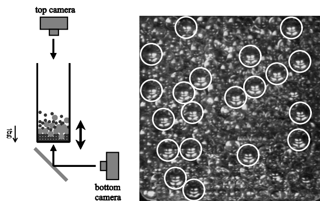
FIG. 1. Left: Experimental setup. The particles are shaken vertically in a square glass tube. Pictures are taken from the top and the bottom (using a mirror) of the granular sample. Right: An image of the bottom plate. All large particles detected by the image processing are marked with white circles.
