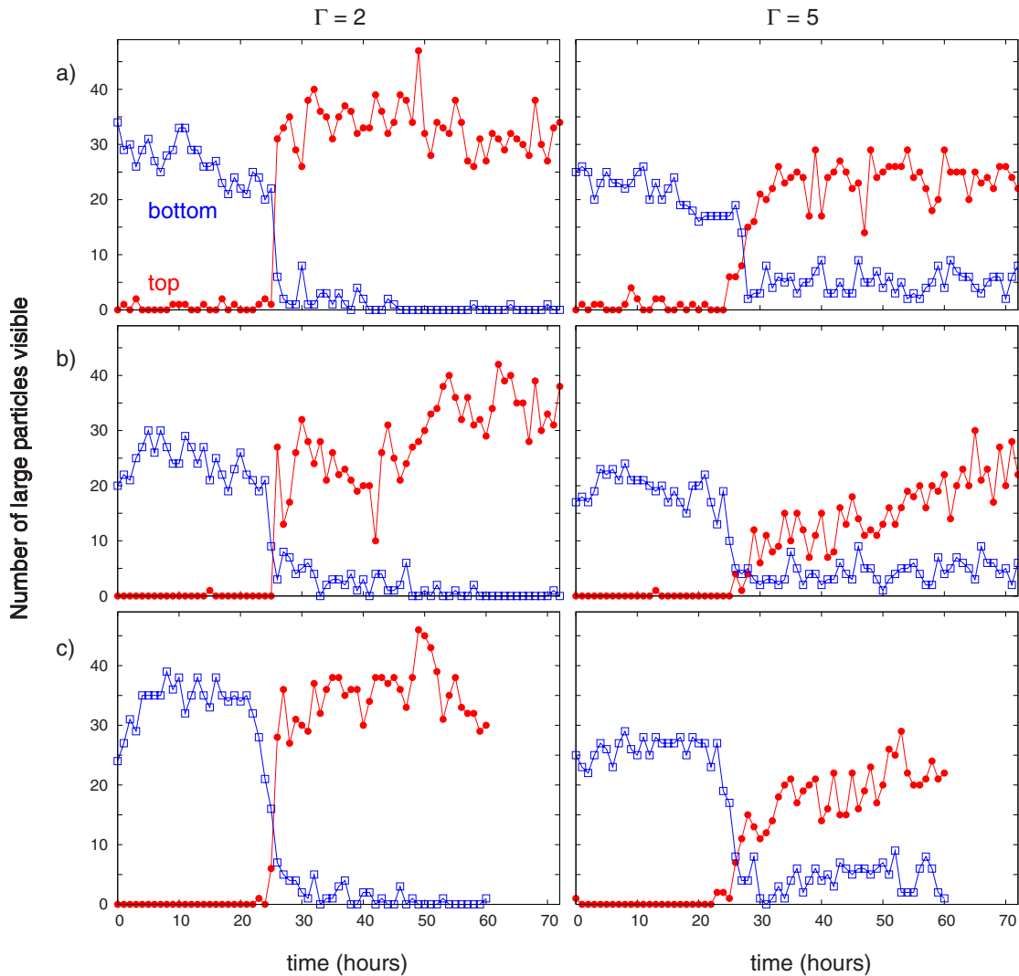
FIG. 2. (Color online) Numbers of large particles at the top and bottom surface of the sample measured at \Gamma = 2 (left column) or 5 (right column). In both cases the segregation changes from a reverse Brazil nut state to a Brazil nut state after about 25 h of aging the particles. Experiment (a) started with new particles; the particles in (b) and (c) were treated in an alkaline ultrasound bath before the start of the experiment. These data were obtained for f = 20 Hz.
