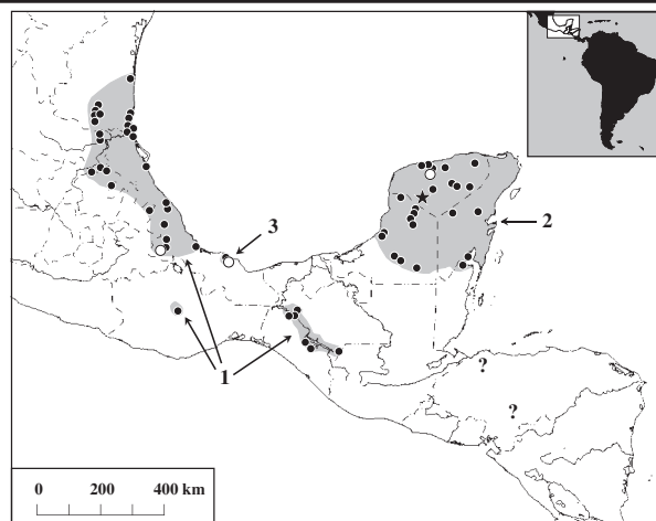
MAP. Distribution of Laemanctus serratus : circles represent type localities and dots indicate other known localities (some dots denote two or more proximate localities). The star indicates a subfossil record tentatively assigned to this species. The two question marks represent probable localities in Honduras (see Remarks ). An old literature record exists for this species (Dugès 1896) for the Mexican state of Guanajuato. We have been unable to locate the purported locality on the maps available to us, but L. serratus may occur in the extreme eastern portion of that state.
