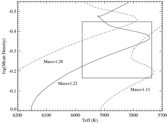
Figure 3. Yonsei–Yale evolutionary tracks for stars with [Z] = 0.17 and masses between 1.13 and 1.28 M_{\odot} , plotted in the \rho_{*} – T_{\text{eff}} plane. The box indicates our adopted observational constraints on \rho_{*} and T_{\text{eff}} . For this range of masses, all tracks lie partly inside the error box, showing that multiple solutions are possible that satisfy these constraints.
