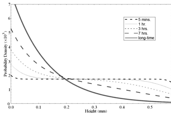
Fig. 2. Plot of P(z,t) versus z for 0.5 \mu\text{m} diameter B-particles in water at t=5 \text{ min} , t=1 \text{ h} , t=3 \text{ h} , t=7 \text{ h} , and the long-time stationary state.
