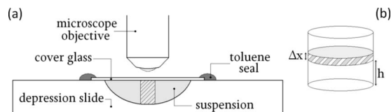
Fig. 3. (a) Experimental setup and the slice of the suspension which we analyzed at varying heights. (b) Note that \Delta x is the focal depth of the microscope, which was 3.04 \mu\text{m} , and h is the height at which the measurement was taken.
