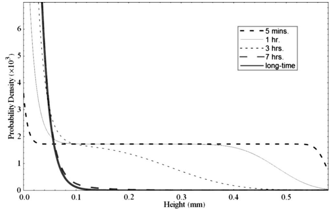
Fig. 1. Plot of the probability density function P(z,t) versus the height z for 1.0 \mu\text{m} diameter B-particles in water at t=5 \text{ min} , t=1 \text{ h} , t=3 \text{ h} , t=7 \text{ h} , and the long-time stationary state.
