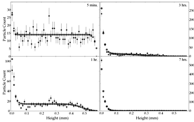
Fig. 5. Experimental data points (black circles with error bars) and predictions of theory (plain black circles) at t=5 min, t=1 h, t=3 h, and t=7 h.
