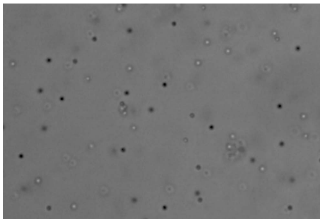
Fig. 4. A picture of 1.0 \mu\text{m} B-particles taken at time t=24 \text{ h} .
