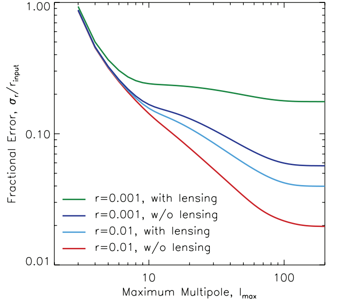
Figure 4. Fractional error, \sigma_r/r_{\text{input}} , on the determination of the value of r as a function of maximum multipoles, l_{\text{max}} . Here, \sigma_r is the square root of the second-order moment of the likelihood function given by Equation (5). (The foreground is not included. Full sky coverage is assumed.) From the top to bottom lines, we show r_{\text{input}} = 0.001 with and without the lensing noise, and r_{\text{input}} = 0.01 with and without the lensing noise, respectively. For the instrumental noise level, we have used 2 \mu\text{K arcmin} . Note that \sigma_r/r_{\text{input}} \sim 1 at l_{\text{max}} = 3 does not mean that we do not detect r ; on the contrary, we detect r with high significance even at l_{\text{max}} = 2 . Rather, it just means that the likelihood for r is highly non-Gaussian and has a long tail toward large values of r (see the top left panel of Figure 3). In other words, we detect r with high statistical significance, but the value of r is not determined very well.
