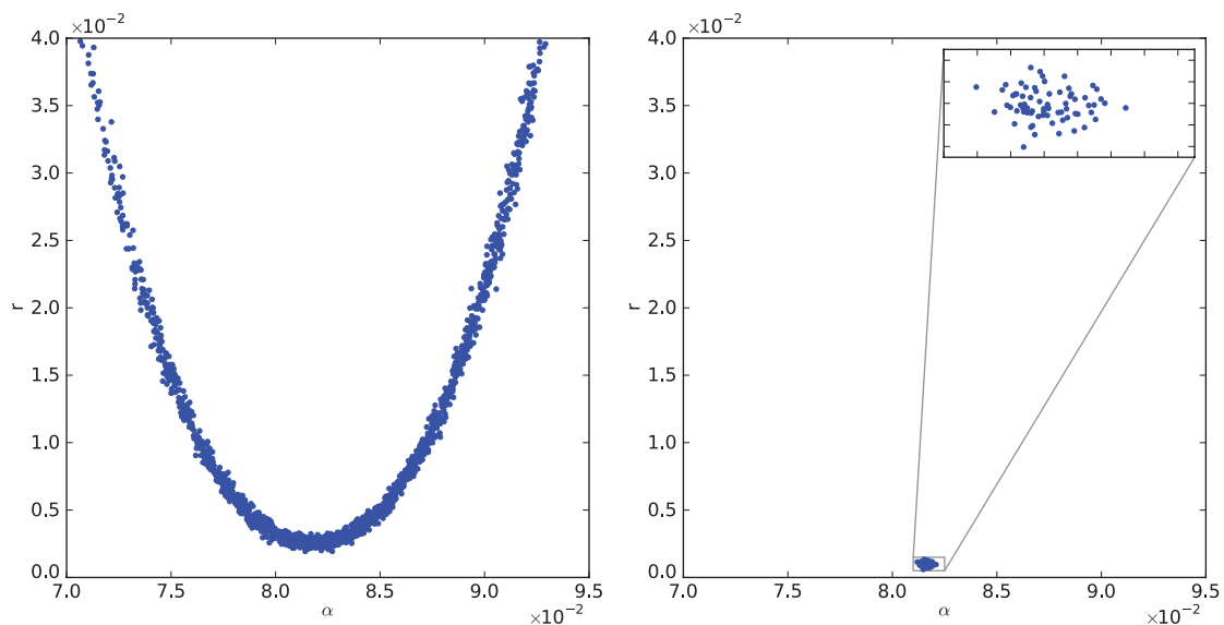
Figure 7. Correlation between the tensor-to-scalar ratio, r , and the amplitude of dust, \alpha_D . Left: the amplitude of the scalar E modes is held fixed at s = 1 . Right: the amplitude of the scalar E modes is treated as a nuisance parameter and marginalized over. The input tensor-to-scalar ratio is r_{\text{input}} = 0.003 and, for this figure only, the original PSM dust map (with an average polarization of \sim 1.5\% ) is used.
