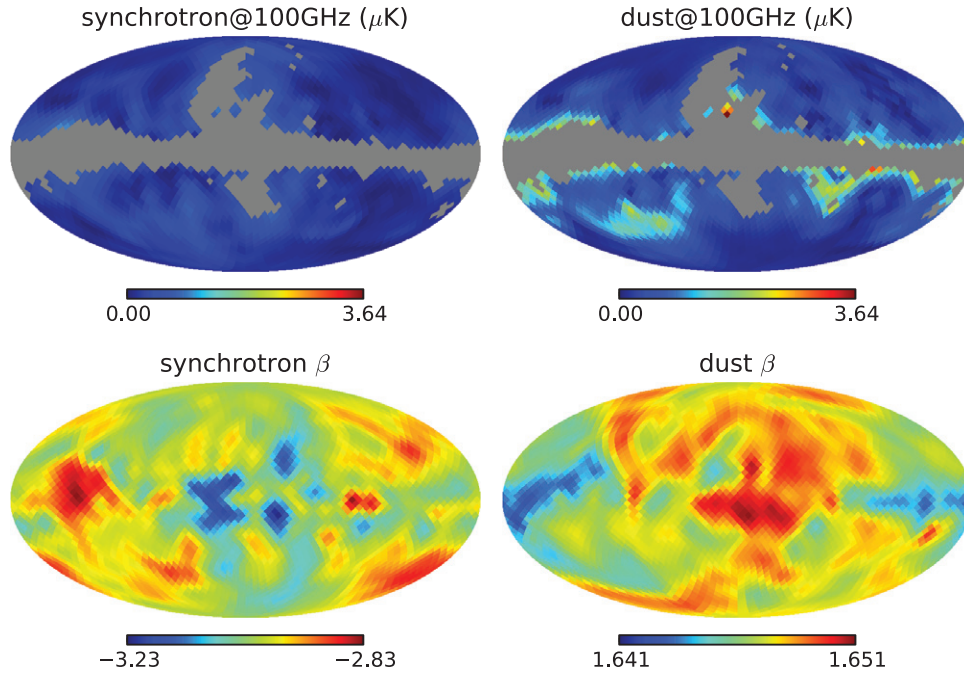
Figure 5. Foreground maps from the Planck Sky Model (PSM; v1.6.2). The top left and top right panels show the polarization intensity maps ( P = \sqrt{Q^2 + U^2} in units of \mu\text{K} ) of synchrotron and dust, respectively. The dust polarization intensity has been multiplied by a factor of three to better approximate a more recent version of PSM. The lower left and lower right panels show the synchrotron index \beta_S and the dust index \beta_D , respectively. Note a small range shown for \beta_D : the dust index does not vary much, but this is a built-in assumption of the PSM v1.6.2.
