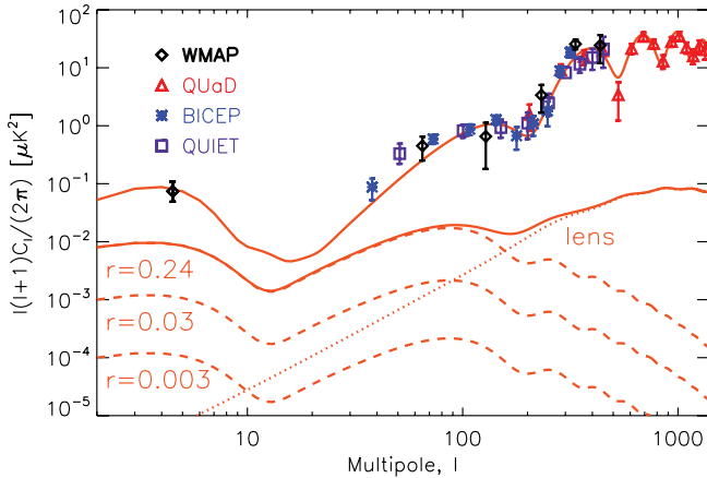
Figure 1. E -mode and B -mode polarization power spectra. The diamonds, triangles, stars, and squares show the WMAP seven-year data (Larson et al. 2011), the QUaD final data (Brown et al. 2009), the BICEP two-year data (Chiang et al. 2010), and the QUIET 43 GHz data ( QUIET Collaboration 2010), respectively. The upper solid line shows the scalar E -mode power spectrum of the WMAP seven-year best-fit model. The dashed lines show the primordial B -mode power spectra with the tensor-to-scalar ratio of r = 0.24 , which corresponds to the current 95% upper limit (Komatsu et al. 2011) as well as of r = 0.03 and 0.003. These lines are linearly proportional to r . The dotted line shows the secondary B -mode power spectrum expected to be generated by the weak gravitational lensing effect converting E modes to B modes (Zaldarriaga & Seljak 1998). This line is fixed (by the WMAP seven-year best-fit model) and acts as noise for the primordial B -mode detection. The lensing contribution becomes comparable to the primordial bump at l = 10 and 100 for r = 0.003 and 0.03, respectively.
