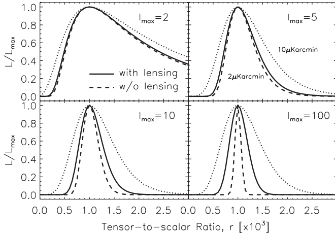
Figure 3. Effect of detector noise and gravitational lensing on the likelihood for r (foreground is not included). The input value of r is r_{\text{input}} = 10^{-3} . The values on the horizontal axis have been multiplied by 10^3 . In the top left, top right, bottom left, and bottom right panels, we sum the multipoles up to l_{\text{max}} = 2, 5, 10, and 100 , respectively. For the detector noise level, we use 2 \mu\text{K arcmin} for the solid and dashed lines and 10 \mu\text{K arcmin} for the dotted lines. The solid and dotted lines include the gravitational lensing contribution to the total noise, while the dashed lines do not. Even if we set the detector noise to be zero, the solid lines do not change very much: for r = 10^{-3} , the gravitational lensing effect prevents us from measuring r accurately beyond l \sim 10 . Note that a single multipole, l = 2 , is enough for us to detect r = 10^{-3} if the detector noise is smaller than 10 \mu\text{K arcmin} .
