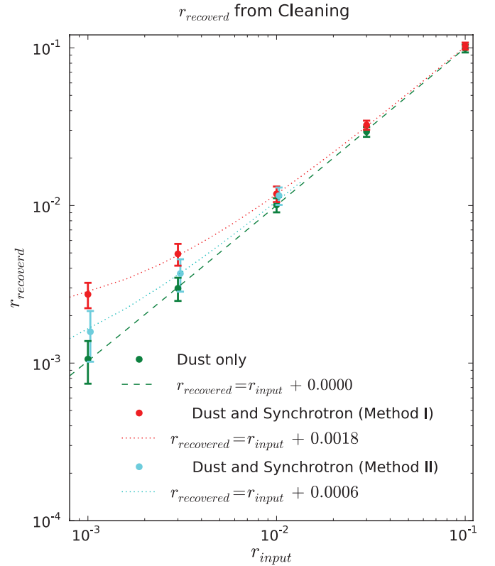
Figure 10. Recovered values of r (mean( r )) and error bars (std( r )) as a function of r_{\text{input}} . The green points with error bars show the recovered r from the dust-only results (Table 1); the red (cyan) points with error bars show the synchrotron-plus-dust results using Method I(II) (Table 3). A systematic bias of \Delta r \approx 0.002(0.0006) is seen for the synchrotron-plus-dust results using Method I(II), which can be described by r_{\text{recovered}} = r_{\text{input}} + (0.0018 \pm 0.0004)(0.0006 \pm 0.0004) (red(cyan) dotted line). We do not detect an offset for the dust-only results: (0.0000 \pm 0.0003) (green dashed line).
