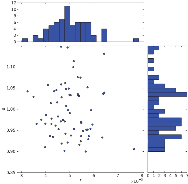
Figure 9. Distribution of r and s obtained from 68 realizations r_{\text{input}} = 0.003 using Method I.
