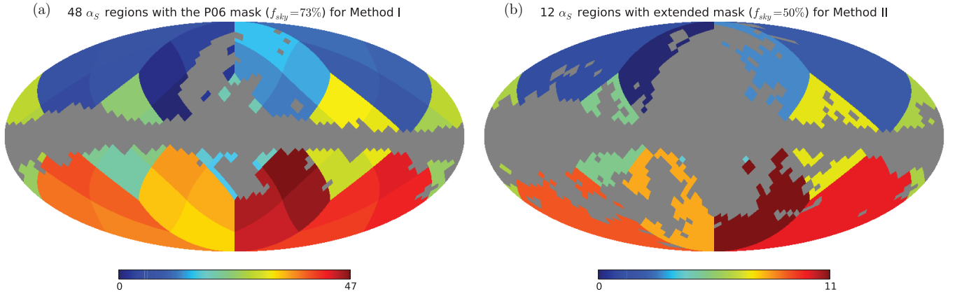
Figure 8. (a) Left: Method I. The P06 masked sky has been divided into 48 regions based on the Healpix map with N_{\text{side}} = 2 . f_{\text{sky}} of the mask is 73%. (b) Right: Method II. The extended-masked sky has been divided into 12 regions based on the Healpix map with N_{\text{side}} = 1 . f_{\text{sky}} of the mask is 50%.
