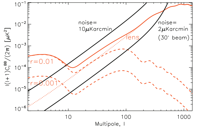
Figure 2. B -mode polarization signal and noise power spectra. The dashed lines show the primordial B -mode power spectra with the tensor-to-scalar ratio of r = 0.01 and 0.001, while the dotted line shows the secondary B -mode power spectrum from gravitational lensing. We also show the noise power spectra (Equation (2)) for w_p^{-1/2} = 2 and 10 \mu\text{K arcmin} with a Gaussian beam window function of \theta_{\text{FWHM}} = 30 arcmin, i.e., N_l^{BB} e^{l^2 \theta_{\text{FWHM}}^2 / (8 \ln 2)} .
