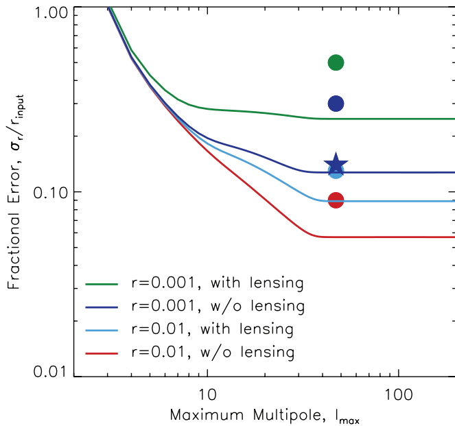
Figure 11. Same as Figure 4, but the foreground-free predictions are made for simulated maps at N_{\text{side}} = 16 (as described in Section 2) and divided by \sqrt{f_{\text{sky}}} , where f_{\text{sky}} = 0.735 for the P06 mask at N_{\text{side}} = 16 . The filled circles use the error bars, \sigma_r , derived from our simulations with synchrotron and dust foreground cleaning (denoted as “std( r )” in Table 3). The denominators, r_{\text{input}} , are not the values recovered from the simulations, but the input values fixed at either 0.01 or 0.001. Each filled circle (foreground-cleaned result from simulations) should be compared to the corresponding line with the same color (foreground-free, analytical prediction). The star shows the foreground-free and lensing-free result from the simulation with r_{\text{input}} = 0.001 , which agrees with the analytical prediction to within 10%.
