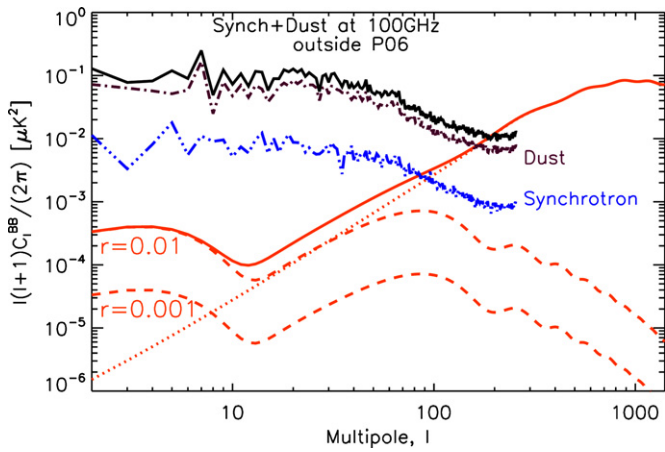
Figure 6. B -mode polarization signal and foreground power spectra. The dashed lines show the primordial B -mode power spectra with the tensor-to-scalar ratio of r = 0.01 and 0.001 , while the dotted line shows the secondary B -mode power spectrum from gravitational lensing. We also show the B -mode power spectra of the dust (dot-dashed line) and synchrotron (triple-dot-dashed line) emission at 100 GHz outside the WMAP P06 mask ( N_{\text{side}} = 128 ). (The measured foreground power spectra have been divided by f_{\text{sky}} = 0.733 to approximately correct for the mask as well as by the pixel window function at N_{\text{side}} = 128 .) The total (synch + dust) power spectrum is measured from the total map, which is slightly larger than the sum of the synchrotron and dust power spectra, as these two foreground components are spatially correlated. Note that the original PSM v1.6.2 dust map has the average polarization fraction of 1.5%, but we have multiplied the dust map by a factor of three to approximate a more recent dust template map adopted by the Planck Collaboration.
