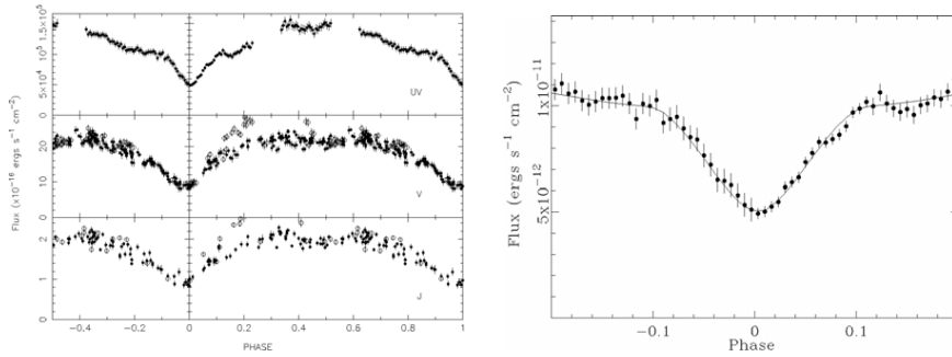
Figure 2. Left Panel: The mean light curve for the integrated UV flux, and the folded V - and J -band light curves. The open circles are from 2005 and the solid circles from 2006. Right Panel: The UV eclipse light curve. The points are the observed light curve and the solid line is the light curve produced by a model with an optically thick toroidal ADC.
