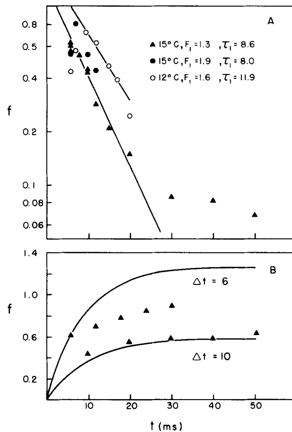
FIGURE 3. (A) Decay of facilitation at 15°C ( \blacktriangle , \bullet ) and 12°C ( \circ ) in a giant synapse of L. pealei . Experimental sequence was 15°C \rightarrow 12°C \rightarrow 15°C ( \bullet ). (B) Summation of facilitation ( \blacktriangle ) during trains of stimuli at intervals of 6 ms ( \Delta t = 6 ) and 10 ms ( \Delta t = 10 ) during the first 15°C experiment above. Solid lines represent growth of facilitation predicted by the linear summation model using F_1 = 1.3 , T = 8.6 from (A). At \Delta t = 6 ms, t = 30 ms, the predictions for f using the power models were 1.46, 1.56, and 1.62 for powers of 2, 3, and 4, respectively. For \Delta t = 10 ms, t = 40 ms, the predictions for f were 0.62, 0.63, and 0.64 for powers of 2, 3, and 4, respectively. (A) and (B) from same synapse. [Ca^{++}]_o = 5 mM, [Mn^{++}]_o = 4 mM.
