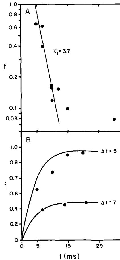
FIGURE 4. (A) Decay of facilitation in an L. pealei giant synapse. F_1 = 2.7 , T_1 = 3.7 . (B) Summation of facilitation in same synapse. Solid lines represent the linear summation prediction. For \Delta t = 5 ms, t = 20 ms, the predictions of the power models were 1.01, 1.04, and 1.06 for powers of 2, 3, and 4, respectively. For \Delta t = 7 ms, t = 21 ms, the predictions of the power models were 0.490, 0.495, and 0.498 for powers of 2, 3, and 4, respectively. (A) and (B) from the same synapse. [Ca^{++}]_o = 6 mM, [Mn^{++}]_o = 2 mM, 19.6^\circ\text{C} .
