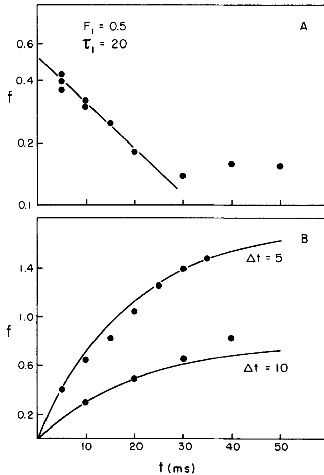
FIGURE 2. (A) Decay and (B) summation of facilitation in an L. brevis non-giant synapse. Solid lines in (B) are the predicted curves from the linear summation model using F_1 = 0.51 , T_1 = 20 found in (A) for stimulus intervals of (lower) 10 ms and (upper) 5 ms. At \Delta t = 5 ms, t = 35 ms, power models predicted that f should equal 1.80, 2.07, and 2.16 for powers of 2, 3, and 4, respectively. At \Delta t = 10 ms, t = 40 ms, the predictions of the power models were 0.72, 0.75, and 0.76 for powers of 2, 3, and 4, respectively. At t = 20 ms, the predictions were 0.50, 0.51, and 0.52. (A) and (B) from the same synapse. [Ca^{++}]_o = 3 mM, 20°C.
