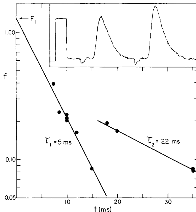
FIGURE 1. Facilitation in a giant synapse of L. brevis . The facilitation ( f ) is plotted using semilogarithmic coordinates against the interval between conditioning and test stimuli ( t ). The first component of facilitation is described by f = F_1 \exp(-t/T_1) , where in this case F_1 (the intercept with the ordinate) = 1.3 and T_1 (the time constant of decay) = 5 ms. Insert shows a plot of a computer average of 20 postsynaptic potentials with an intrapulse interval of \sim 10 ms. Calibration pulse: 2mV, 2 ms. [Ca^{++}]_o = 4 mM, 18°C.
