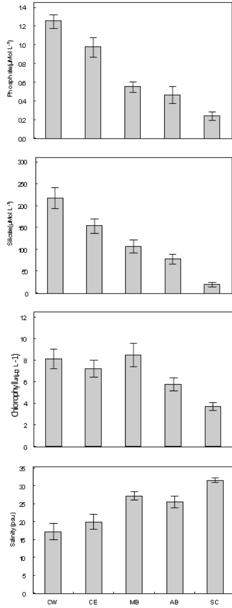
Figure 7.2. Nutrient concentrations and salinity of Mission-Aransas NERR SWMP stations. Data represent mean values from 2007-2009 monthly samples. Error bars represent standard error. CW=Copano Bay West, CE=Copano Bay East, MB=Mesquite Bay, AB=Aransas Bay, SC=UTMSI pier.
