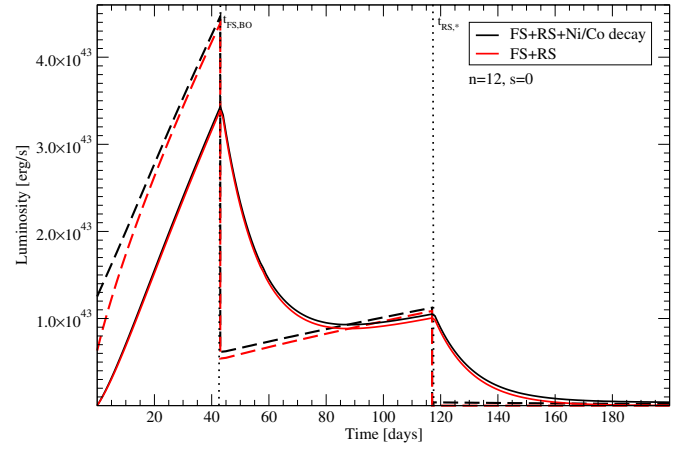
Figure 6. Comparison of SN ejecta–CSM interaction and hybrid SN ejecta–CSM interaction plus ^{56}\text{Ni} and ^{56}\text{Co} radioactive decay LC models for the case of collision with a constant density CSM shell ( n = 12 , s = 0 ). The hybrid forward, reverse and ^{56}\text{Ni} and ^{56}\text{Co} radioactive decay model is shown in black and the pure forward and reverse shock ejecta–CSM interaction model in red. In each case, the dashed curve represents the input luminosity and the solid curve the output LC model. The dotted vertical lines indicate the forward shock breakout time (essentially equal to the time of termination of forward shock input in the optically thick part of the CSM) and the reverse shock termination timescale. The forward termination timescale is very close to its breakout timescale in the case of a CSM constant density shell. The models were drawn for the following choice of parameters: \delta = 0 , E_{\text{SN}} = 10^{51} erg, M_{\text{ej}} = 12 M_{\odot} , M_{\text{CSM}} = 1 M_{\odot} , R_p = 10^{14} cm, \rho_{\text{CSM},1} = 10^{-13} g cm ^{-3} , and M_{\text{Ni}} = 0.08 M_{\odot} . (A color version of this figure is available in the online journal.)
