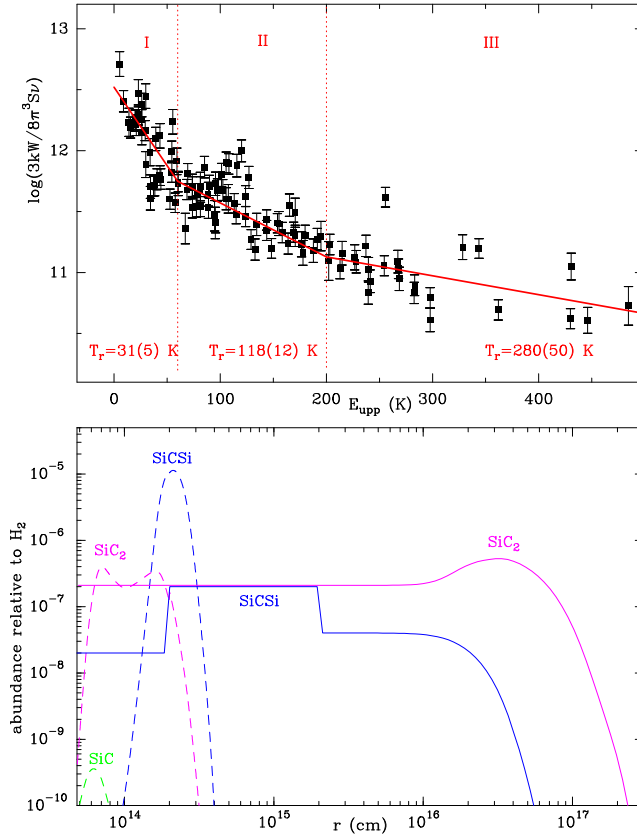
Fig. 3.— The top panel shows the rotational diagram of the 112 observed lines of SiCSi. The three zones discussed in the text are indicated by vertical dashed lines. The bottom panel shows the radial abundance distribution of SiCSi, SiC 2 , and SiC as calculated by chemical equilibrium (dashed lines) and as derived from the observations of IRC +10216 (solid lines). The derived abundance profile of SiC 2 is taken from Cernicharo et al. (2010).
