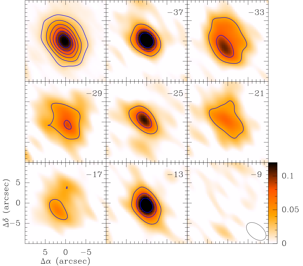
Fig. 2.— Maps of the average of four SiCSi lines: 18_{3,15} - 18_{2,16} , 16_{3,13} - 16_{2,14} , 14_{3,11} - 14_{2,12} and 12_{3,9} - 12_{2,10} (from the SMA line survey of IRC +10216 Patel et al. (2011)). Their visibilities were combined before imaging. The upper left panel is the integrated intensity map, while the remaining ones are the channel maps with V_{\text{LSR}} velocities indicated on top right in \text{km s}^{-1} . The size of the synthesized beam is shown in bottom right panel. The halftone image in the first panel is scaled linearly from 0 to 2.7 \text{ Jy beam}^{-1} \text{ km s}^{-1} and the contour levels (in the same units) have the starting value and intervals of 0.4 in the first panel and 0.04 in remaining panels.
