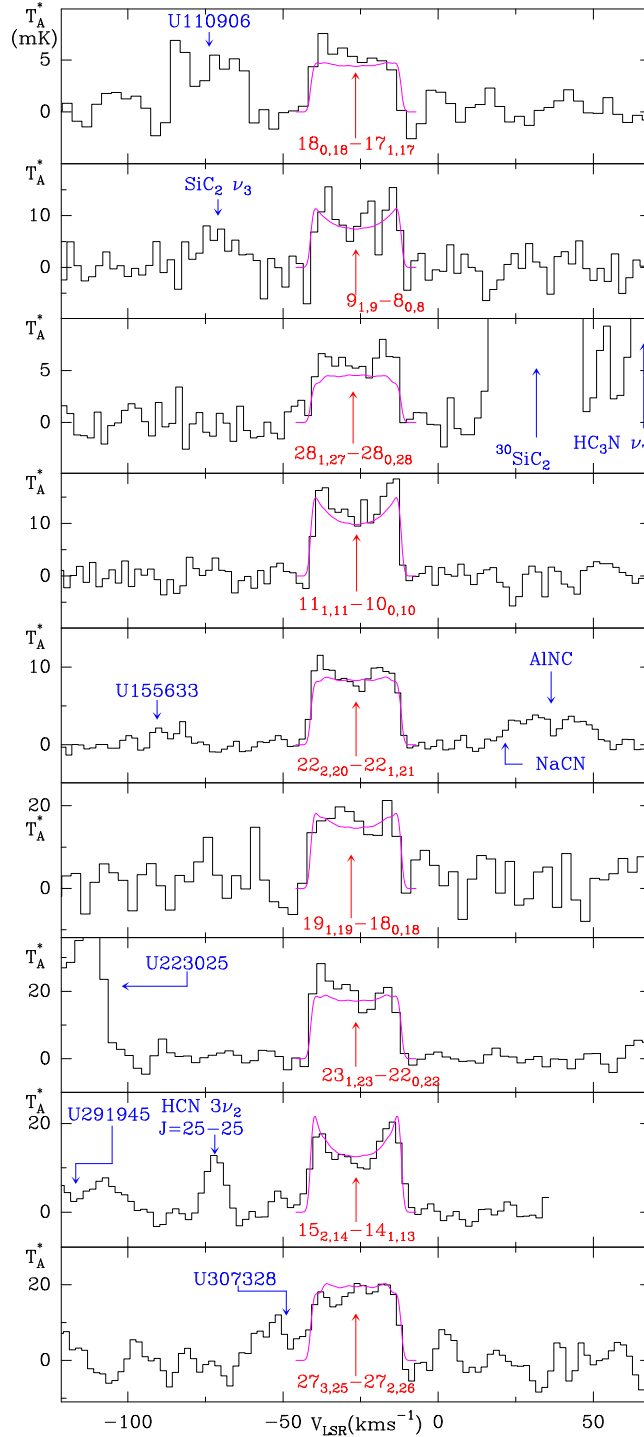
Fig. 1.— Selected transitions of SiCSi among the 112 observed lines. Unidentified (U) lines are indicated by their frequency in MHz. The intensity scale is antenna temperature in mK. The data are shown as histograms. Violet continuum lines show the predicted line profile from the best model for the abundance of SiCSi (see text).
