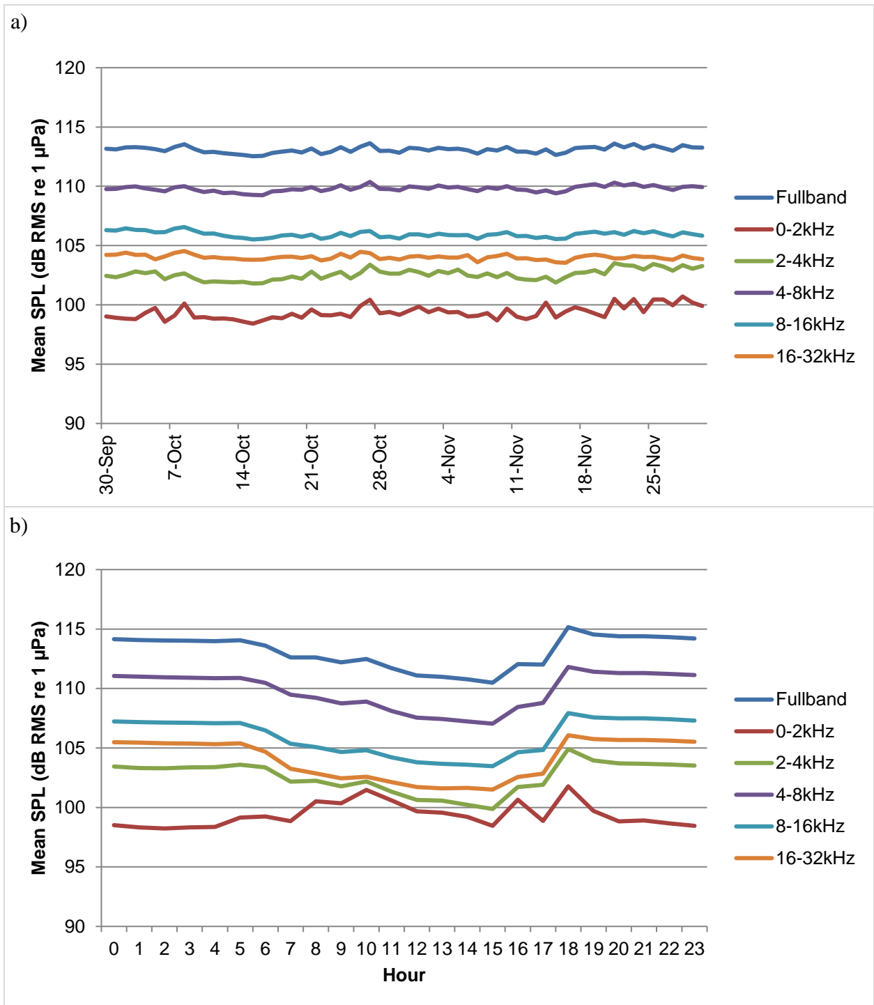
Figure A7. Mānele fall deployment root mean square sound pressure level in 1-octave frequency bands by date from 30 September 2016 to 30 November 2016 (a) and by hour of day from 0000 to 2300 h (b)
