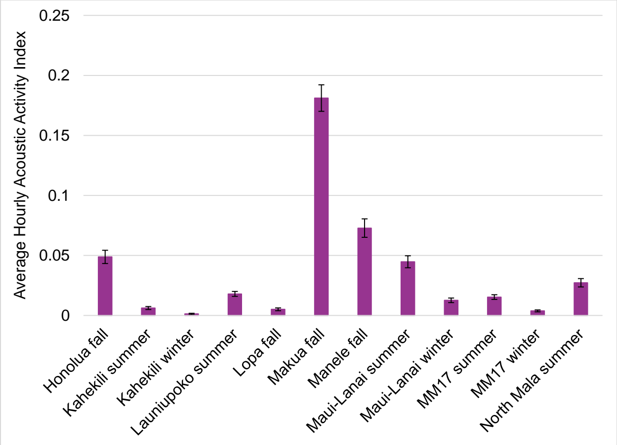
Figure 2. Average hourly AAI ( \pm SEM) in each deployment. Deployments are denoted by location and season in which they took place.
