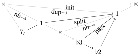
Figure 6: An analysis of the phrase in Figure 2 using the rāga grammar. Dark edges indicate the subgraph induced by removing non-note nodes ( \times , \bar{\times} , \varepsilon ).
