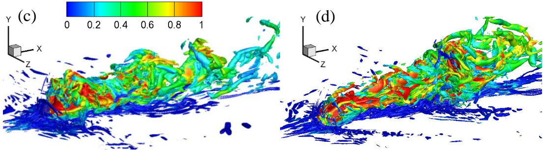
Fig. 5. Numerical Schlieren \|\nabla\bar{\rho}\| of different instants in the central plane ( z/D=0 ) and the three-dimensional instantaneous vorticity field in terms of the Q-criterion isosurface ( Q=10^{11} ) coloured by H2 mixture fraction, (a & c): single injection, (b & d) two-stage injection.
