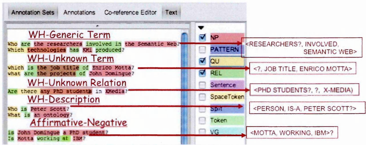
Figure 5.1 Screenshot example of GATE annotations and Query-Triples for basic queries
