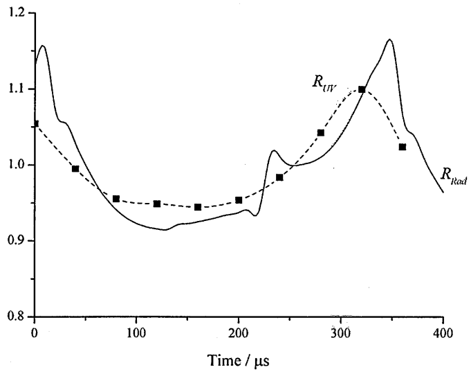
Figure 4.9: A comparison of the normalised radial variation measured from the UV and modelled emission for a modulation depth of 22 % (top) and 33 % (bottom).
