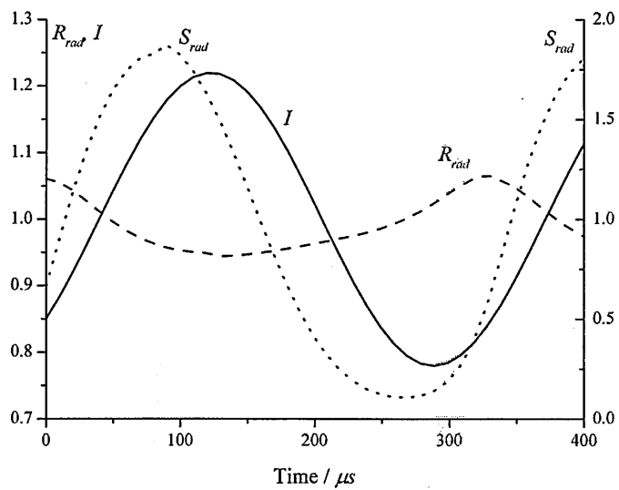
Figure 4.8: Upper graph shows the measured data of the UV emission repeated from figure 4.7. Normalised variation of the discharge radius (dash), modulating current (solid) and optical intensity (dots) for 3 kHz modulation calculated from the model; z = 6 mm, modulation depth = 22 % (lower).
