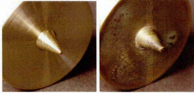
Figure 3.15: The ground electrode (left) and eroded electrode with surface damage around the electrode base (right).
