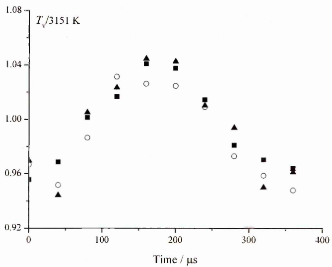
Figure 4.12: T_r (top) and T_v (bottom) variation at r = 0\text{mm} (Square), 0.5 \text{ mm} (circle) and 1 \text{ mm} (triangle); z = 0.5 \text{ mm} .
