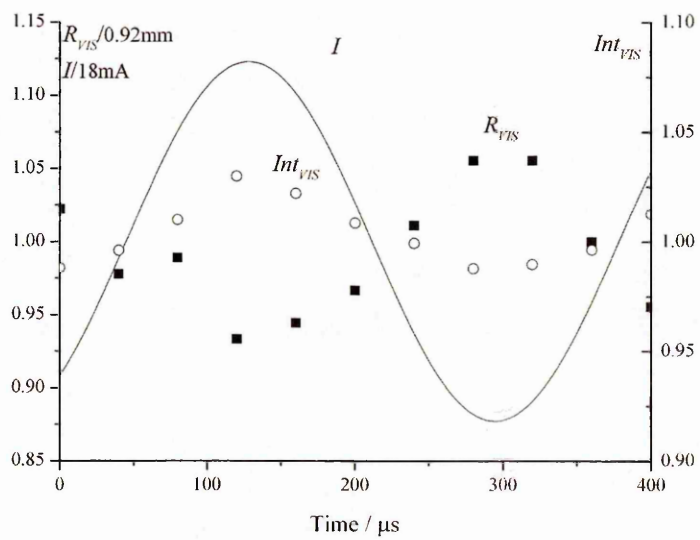
Figure 4.6: Normalised variation of the discharge radius (square), modulating current (solid) and optical intensity (circle) determined from the UV emission (top) and visible emission (bottom); z = 6 \text{ mm} ; rms conduction current = 18 mA.
