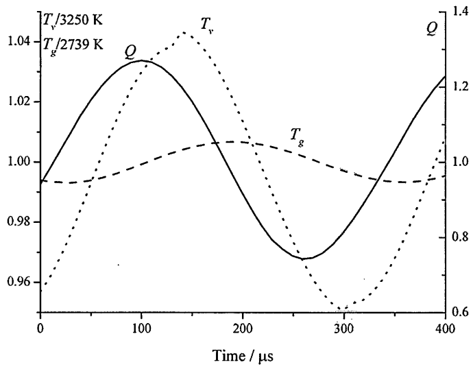
Figure 4.13: Modelled temperatures and power for a modulation depth of 22 % at z = 6 mm (top) and z = 0.5 mm (bottom).
