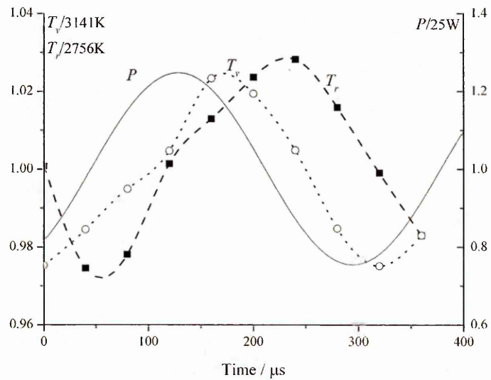
Figure 4.10: Measured temperatures and power for a modulation depth of 22% at z = 6 \text{ mm} (top) and z = 0.5 \text{ mm} (bottom).
