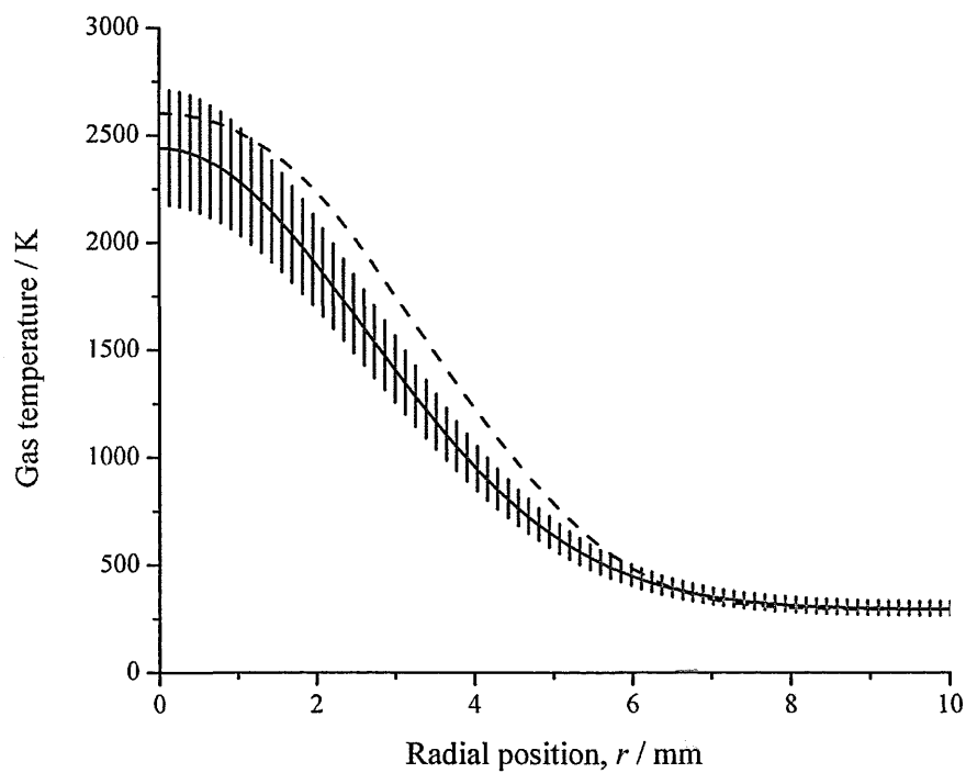
Figure 5.30: Radial (Schlieren) gas temperature (solid) and modelled gas temperature profile (dashed) at axial positions z = 6 mm (top) and 10 mm (bottom) and for an rms conduction current of 18 mA.
