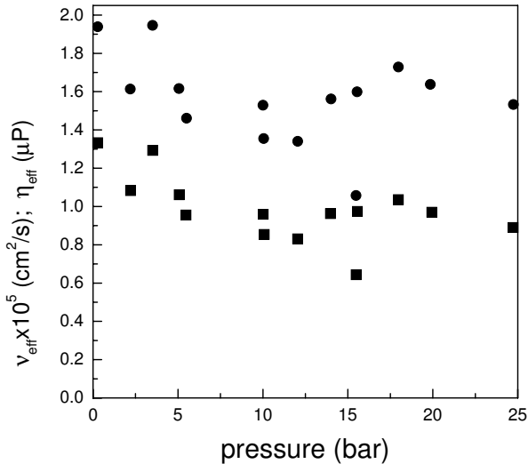
FIG. 12: Calculated values of the effective kinematic viscosity (squares) and dynamic viscosity (circles) versus pressure.
