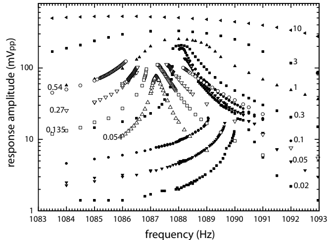
FIG. 11: Resonance curves measured at 3.5 bar using the memory oscilloscope for drive levels (in V_{\text{pp}} ) as indicated. Filled symbols represent the regular grid behaviour obtained with the “cleaned” grid, while the virgin behaviour is represented by resonant curves composed of the open symbols. The upper three curves plotted with open symbols are shown up to the drive amplitude at which the onset of beating occurred (see text).
