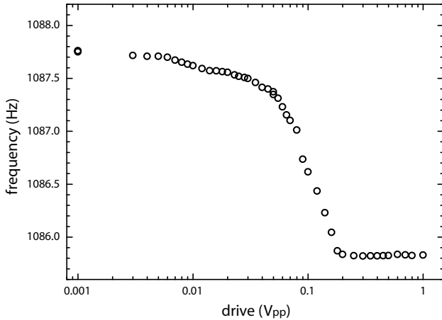
FIG. 7: The drive dependence of the resonance frequency measured at 10 bar using the lock-in amplifier.
