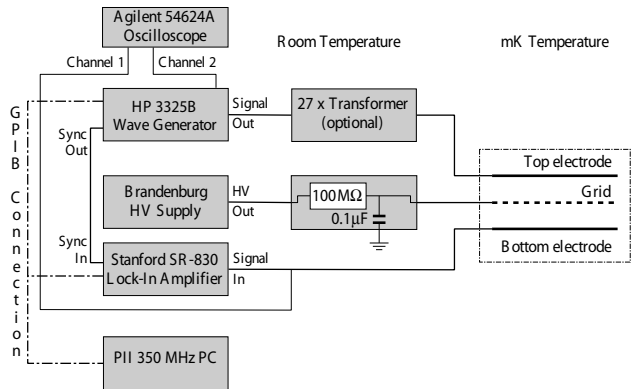
FIG. 3: Schematic block diagram of the experiment, showing the main components used for the measurements.
