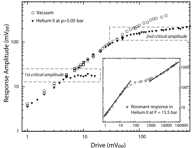
FIG. 6: Response amplitude of the grid versus the drive level at resonance measured in vacuum (open symbols) and in He II at p = 5.05 bar (main figure). The positions of the first and the second thresholds are indicated in order to emphasize that above the first threshold the damping remains unchanged, provided the measurements are recorded in sequence from high-drive towards low-drive. The inset shows the drive dependence of the response amplitude of the grid at p = 15.5 bar, indicating regions of laminar and turbulent flow regimes. The full lines indicate the linear and square-root responses.
