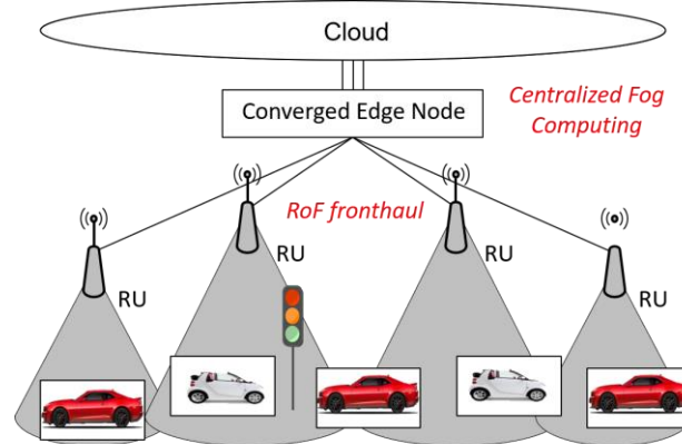
Fig. 6: A simple, converged fiber/wireless edge node, which facilitates realtime processing of live traffic data.
