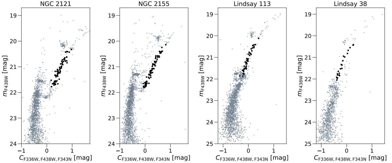
Figure 5. C_{F336W, F438W, F343N} vs. m_{F438W} CMDs for the clusters analysed in this paper. Black circles indicate the final selected RGB stars.
