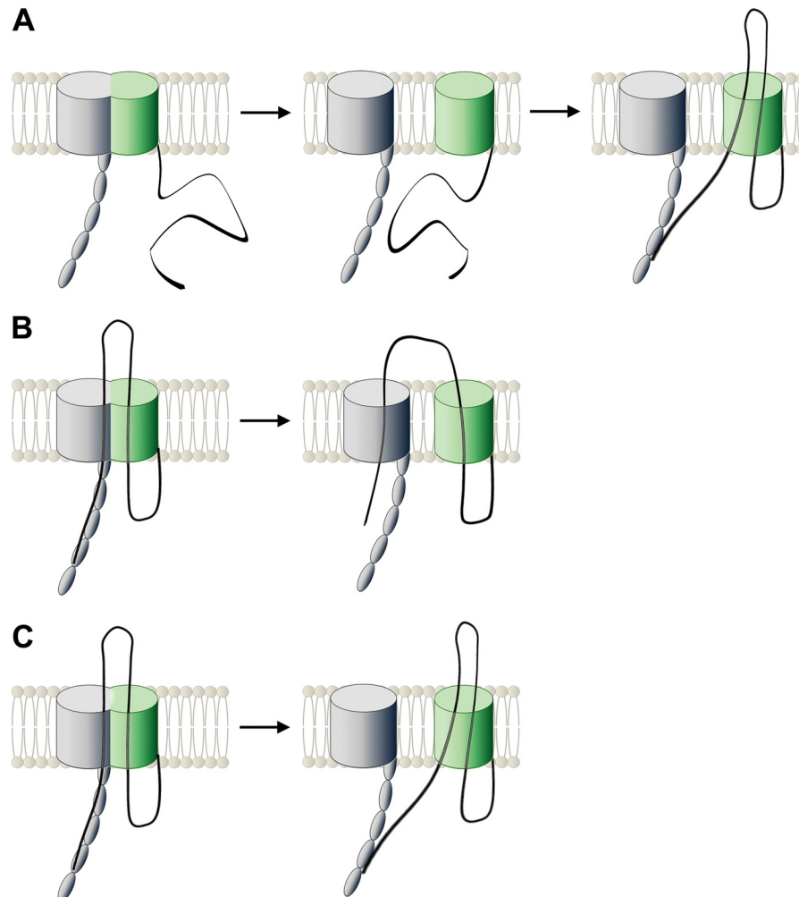
FIGURE 10. Possible scenarios explaining our findings. A , during the first step of biogenesis, the intimin barrel and the BamA \beta -barrel build a hybrid barrel from which the intimin barrel buds off into the OM. Then autotransport of the passenger is initiated and is halted due to the presence of the HA tag in a hairpin conformation. Direct contact with BamA at this stage is maintained either via interaction of the passenger with POTRA domain(s) or via the folded \beta -barrels. B and C , intimin biogenesis is initiated by the formation of a hybrid barrel with BamA. At this hybrid barrel stage, the hairpin is inserted. Budding of the intimin barrel can lead to two outcomes; the passenger stays in the BamA-barrel and mediates contact to the barrel wall ( B ), or the passenger ends up in the intimin barrel ( C ). Contact with BamA is then mediated either via the POTRA domain(s) or by interaction of the intimin and the BamA \beta -barrel domains.
