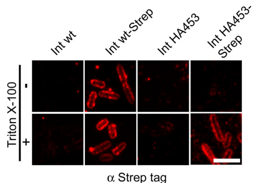
FIGURE 6. Immunofluorescence staining of C-terminally Strep-tagged IntHA453 AT intermediate indicates a hairpin conformation of the passenger domain. Int WT or IntHA453 as well as Strep-tagged variants were expressed in E. coli BL21(DE3)omp2. Bacterial outer membrane was permeabilized (bottom) or not (top) with Triton X-100 prior to staining with anti-Strep-tag primary antibody. Scale bar, 5 \mu m.
