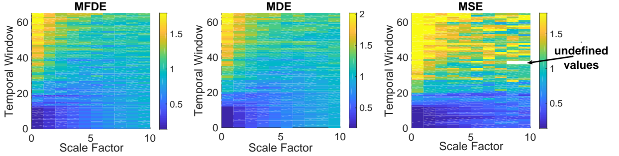
Fig. 8: Mean value and SD of the MFDE, MDE, and MSE results for the quasi-periodic time series with increasing additive noise power using a window moving along the signal (temporal window). The MSE values at several temporal scale factors are undefined.
